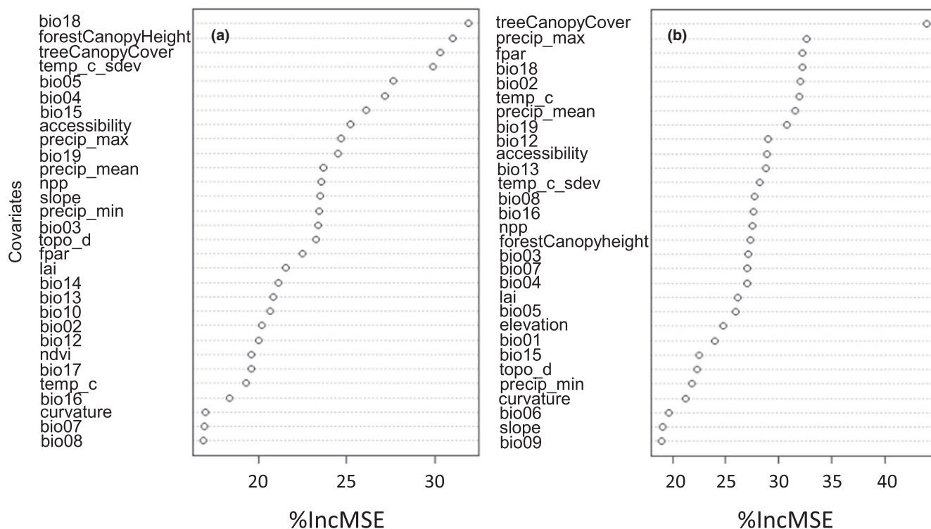
FIGURE 2 Covariate importance for selected target variables (a) tree height and (b) tree density based on the percentage increase in mean squared error (%IncMSE).
