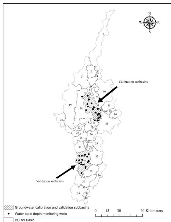
Figure 3. Watershed map showing groundwater monitoring wells, model calibration, and validation subbasins.
