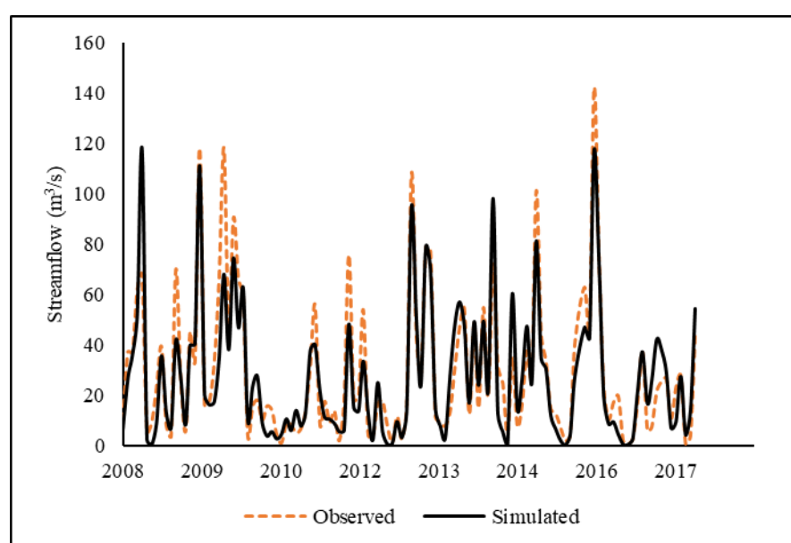
Figure 5. Simulated and measured streamflow during calibration and validation at Sunflower gauge station.
