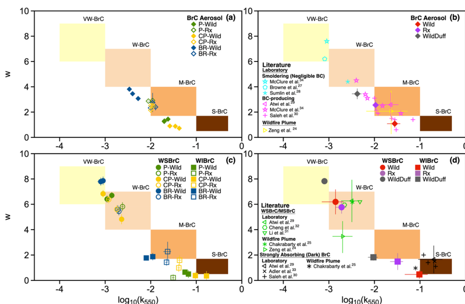
Figure 3. Light-absorption properties of BrC aerosol, WSBrc, and WIBrc from all experiments plotted in \log_{10}(k_{550})-w space. The shaded regions represent the optical classes proposed by Saleh: 15 very weakly absorbing BrC (VW-BrC), weakly absorbing BrC (W-BrC), moderately absorbing BrC (M-BrC), and strongly absorbing BrC (S-BrC). Error bars represent uncertainty, calculated as described in the SI. Numerical values of each of the data points are given in SI Table S4. (a) BrC aerosol for each of the six experimental permutations. (b) Averages of the data points in panel (a) for the three groups: wild, Rx, and WildDuff. Also shown are values calculated from data obtained from previous studies. Numerical values of each data point and information on how k_{550} and w were calculated from each study are given in SI Table S5. (c) WSBrc and WIBrc for the six experimental permutations. (d) Averages of the data points in panel c for the three groups: wild, Rx, and WildDuff. Also shown are values calculated from data obtained from previous studies for WSBrc and methanol-soluble BrC (MSBrC) and strongly absorbing (dark) BrC. Numerical values of each data point and information on how k_{550} and w were calculated from each study are given in SI Table S5.
