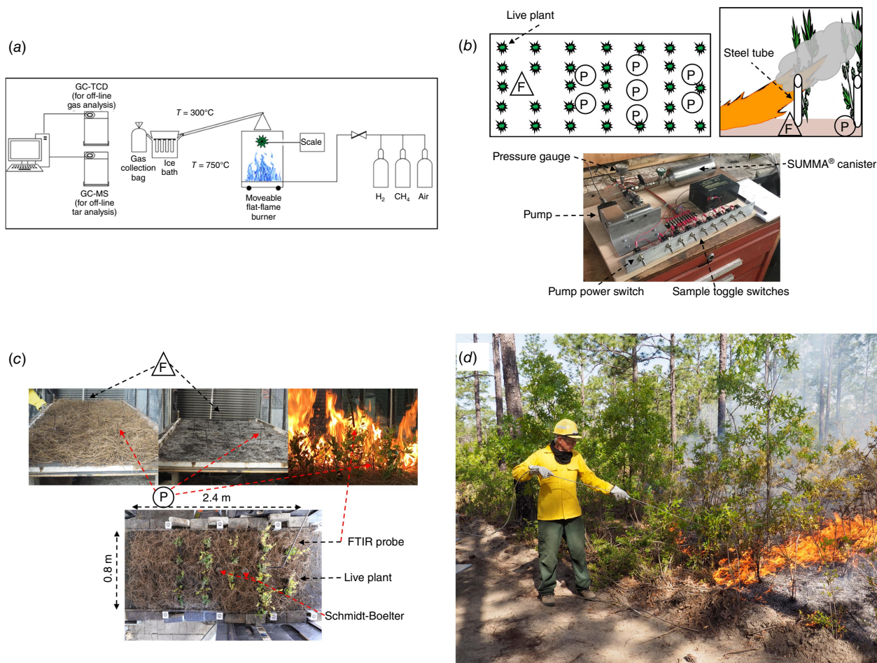
Fig. 1. Experimental setups to determine composition of fast pyrolysis gases in non-oxidising (a) and oxidising (b–d) environments. (a) Flat-flame burner setup used to heat southern U.S. wildland fuels in an O_2 -free (fuel rich) post-flame environment. (b) canister sampling for flaming (F) and pyrolysis gases (P) in a wind tunnel where the fire's flame heated fuels. (c) FTIR and GC/FID sampling setup in the wind tunnel. (d) canister sampling for FTIR and GC/FID in the field.
