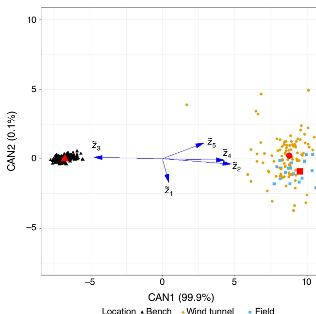
Fig. 4. Plot of first two dimensions resulting from canonical discriminant analysis (CDA) stressing the difference in scientifically meaningful balances (Table 1, \tilde{z}_k ). between the oxidising (wind tunnel, field) and non-oxidising environments (bench). These two dimensions accounted for 100% of original variability. Arrows indicate the balances that separated the two environments. Points indicate CDA scores of the original observations. The large red symbols indicate the mean values of the CDA scores for each group. Field = 0.1 ha prescribed burn plots, Ft. Jackson, SC, US.
