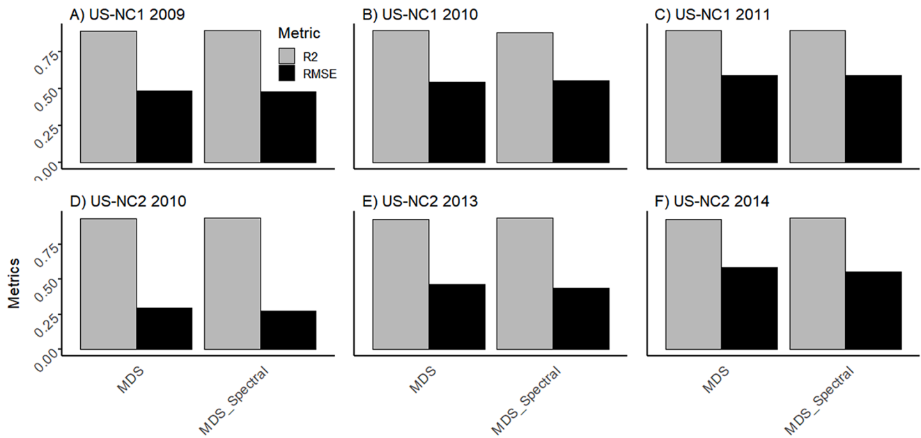
Fig. 2. Bar plot summarizing statistical model performance (quantified by R^2 , RMSE) of soil respiration ( R_s ) gapfilling using two different variants of the Marginal Distribution Sampling algorithm, employing two distinct sets of environmental inputs for model calibration: measured data (MDS) and spectrally filtered data (MDS_Spectral).
