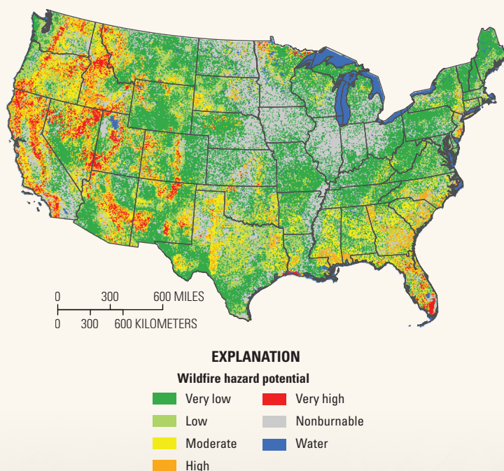
Figure 1. Wildfire hazard based on LANDFIRE 2014 fuels and topography.
