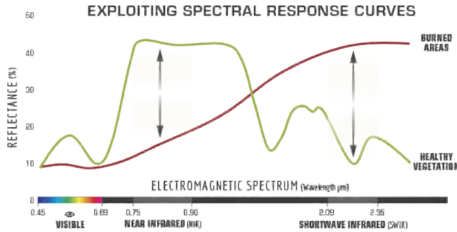
Figure C4. The normalized burn ratio uses the difference in reflectance for the near-infrared and shortwave infrared parts of the electromagnetic spectrum for healthy vegetation as compared to burned areas. Image courtesy of Wasser and Cattau (2022), licensed under the Creative Commons Attribution-Share Alike 4.0 International license. [%, percent; \mu\text{m} , micrometer]
