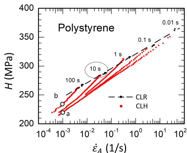
Fig. 2. Indentation creep of polystyrene from 11 based on \dot{\epsilon}_A , suggesting path-dependent behavior based on constant loading rate (CLR) and constant load hold (CLH). A close-up of the 10-s loading data is given in Fig. 3.
