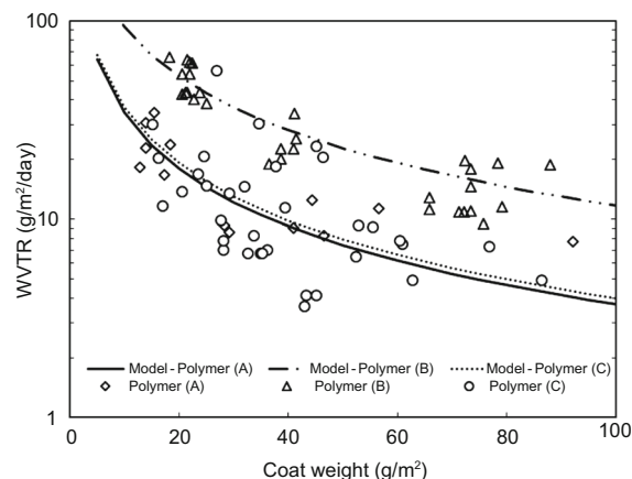
Fig. 5: WVTR for the three polymers with no barrier pigments. Lines are a fit of equation (1) through the data minimizing the root mean square error
