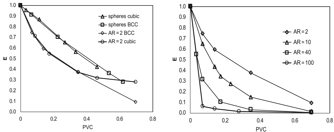
Fig. 11: The influence of PVC on the effectiveness parameter for cubic packed spheres, BCC packed spheres, and BCC packed disks with an aspect ratio (AR) of 2 (left) and as a function of pigment volume concentration for BCC packed disk-shaped particles for aspect ratios of 2, 10, 40, and 100 (right)
