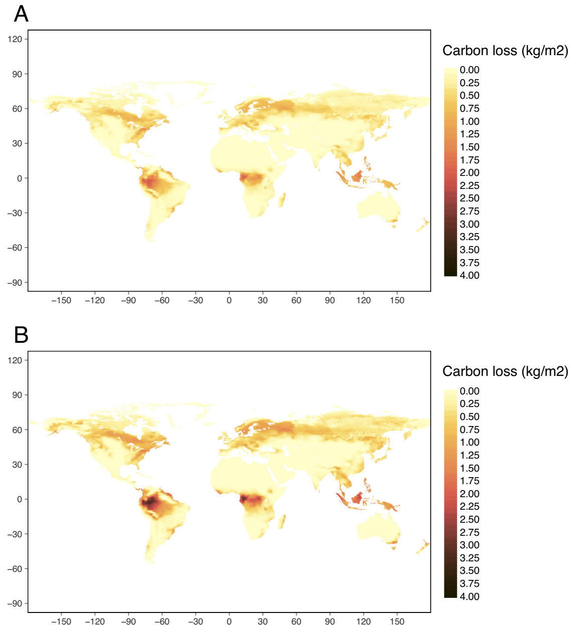
Fig. 3 | Carbon loss by ecoregion. Carbon loss ( \text{kg/m}^2 ) driven by long-term loss of plant biodiversity by ecoregion under a global sustainability (SSP1/RCP2.6, A ) and fossil-fueled development (SSP5/RCP8.5, B ) scenario using the mean biodiversity-ecosystem functioning slope b = 0.26 and a species-area relationship z = 0.25 . Darker areas indicate greater carbon loss. This carbon loss is from within remaining
