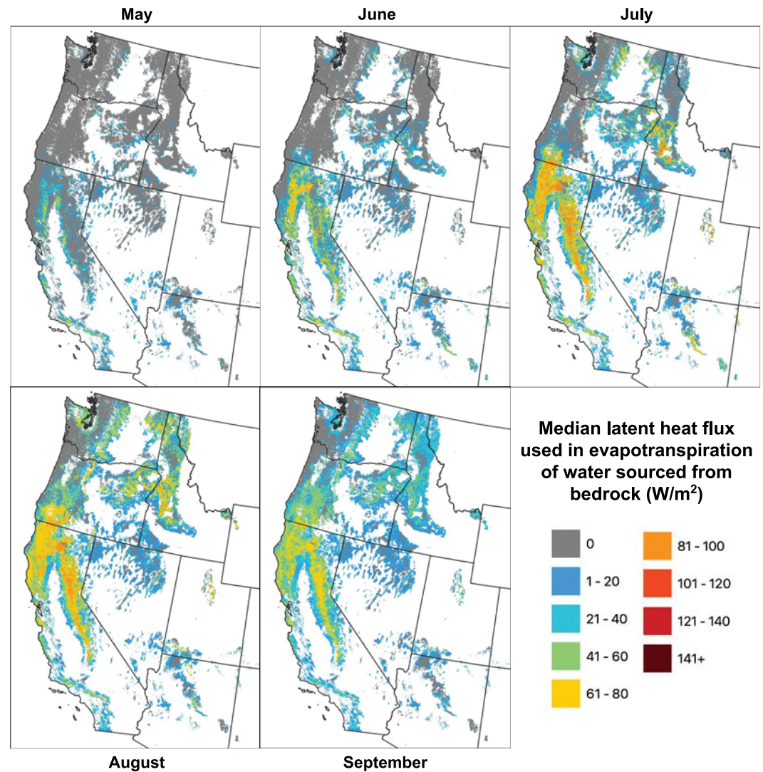
Figure 7. Median latent heat flux (equivalent units to solar irradiance, \text{W/m}^2 ) used in evapotranspiration that is sourced from S_{\text{bedrock}} during the growing season. In large parts of the western US, in particular northern California and the Sierra Nevada mountain ranges, a large latent heat flux is associated with evapotranspiration of bedrock water every summer.
