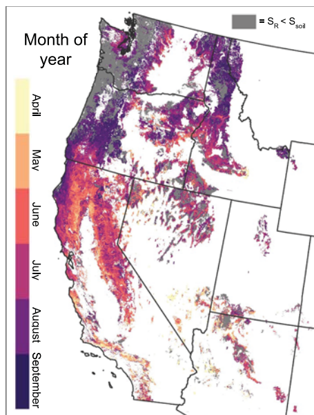
Figure 5. Typical month in which the annual root-zone storage deficit ( S_R ) exceeds the soil water storage capacity ( S_{\text{soil}} ), implying plant transpiration beyond this point must be using S_{\text{bedrock(my)}} to sustain transpiration and growth. Bedrock water is accessed very early into the growing season for many parts of the western US.
