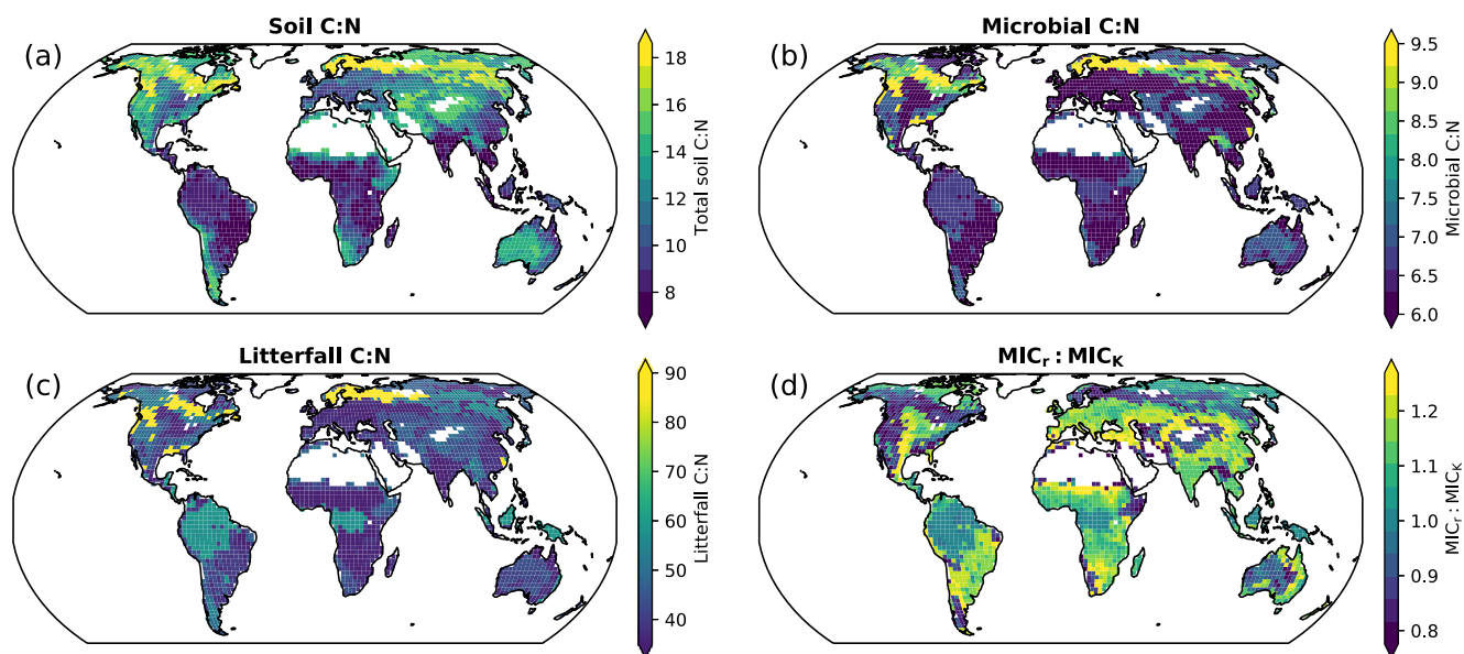
Figure 4. Spatial distribution of mean (a) soil C:N, (b) microbial biomass C:N, (c) litterfall C:N, and (d) the relative abundance of MIC_r:MIC_k that were simulated by the Microbial-Mineral Carbon Stabilization-carbon-nitrogen model at initialization (1901–1920).
