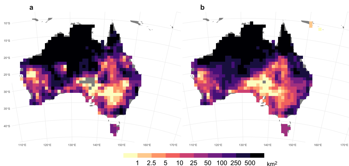
Fig. 4 Mean annual burned area (km 2 ) for the ONFIRE (panel a) and the FireCCI51 (panel b) datasets for Australia. Data for the period 2001–2020, or shorter depending on the data availability (see Tables 1, 2). Areas with no data are shown in grey.
