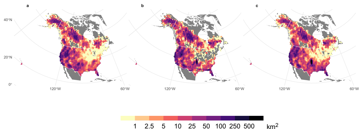
Fig. 3 Mean annual burned area (km 2 ) averaged over the period 2001–2020 using data from various sources for Canada and the U.S.A. The different panels show the results obtained by combining different data sources: (a) ONFIRE-NBAC for Canada and ONFIRE-FPA-FOD for the U.S.A.; (b) ONFIRE-NFDB for Canada and ONFIRE-MTBS for the U.S.A.; (c) FireCCI51. Areas with no data are shown in grey.
