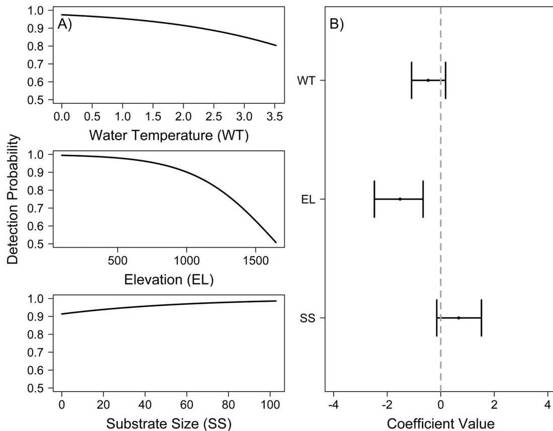
Fig. 3. Channel catfish Ictalurus punctatus mitochondrial environmental DNA (eDNA) (A) detection probabilities and (B) parameter estimates in relation to water temperature (°C), elevation (m), and modal substrate size (mm). Parameter estimates with 90% credibility intervals that intersect the reference line at 0 are not strongly supported
