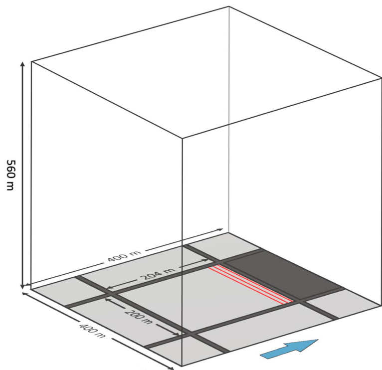
Fig. 2 Computational domain design showing areas with surface fuels (light gray), areas where surface fuels have been removed (dark gray), and the three initial fire lines (red). The arrow shows the streamwise wind direction, pointing towards the direction wind is going (blue). The area of interest (AOI) for this simulation is the light gray area (204 m × 200 m × 560 m) in the center of the domain
