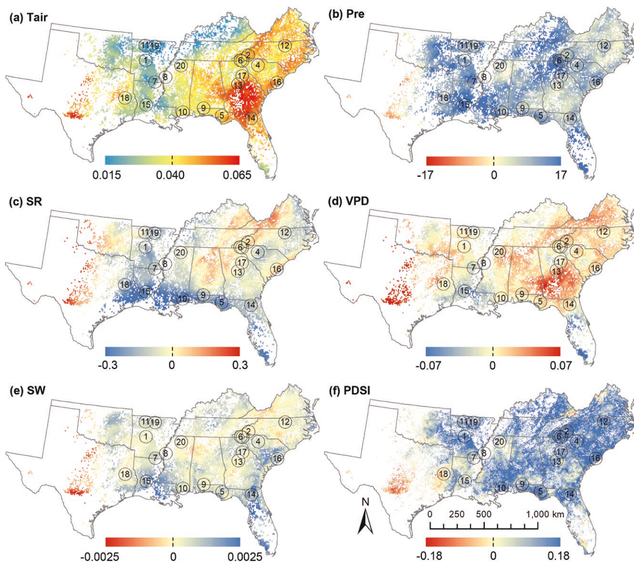
Figure 5 Long-term trends of annual (a) temperature (Tair; °C yr -1 ), (b) precipitation (Pre; mm yr -1 ), (c) shortwave solar radiation (SR; W m -2 yr -1 ), (d) vapor pressure deficit (VPD; hPa yr -1 ), (e) volumetric soil water content (SW; % yr -1 ), and (f) PDSI from 2001 to 2022 for the southeastern forest region. The numbers in circles stand for experimental forests and ranges (EFRs); the correspondence between the numbers and the EFRs is provided in Table 1.
