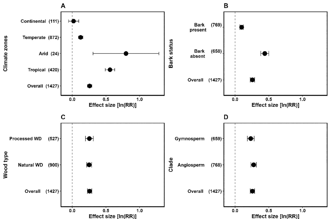
Fig. 2. Invertebrate effect on woody debris (WD) decomposition across climate zones (A), bark status (B), WD type (C), and WD clade (D). Effect sizes with error bars crossing zero (vertical dashed line) are not significantly different from zero. Numbers in parentheses are the number of observations.
