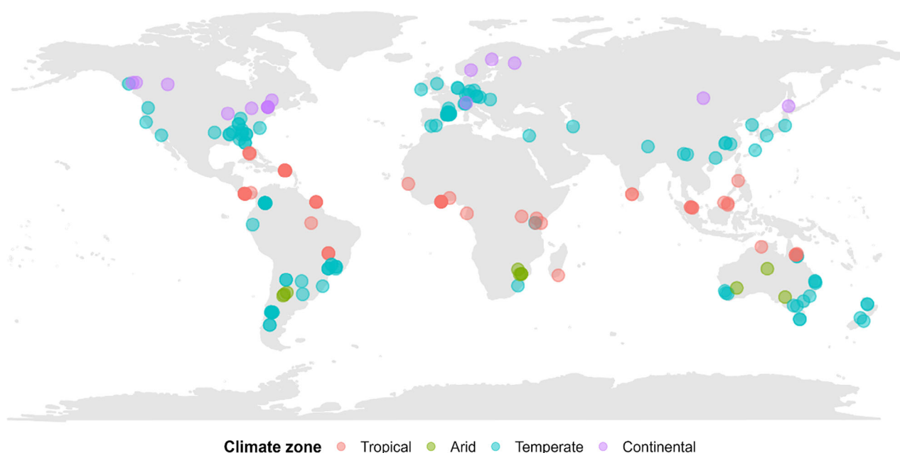
Fig. 1. Study site geographical distributions. The climate zones are based on the Köppen Geiger climate classification, which recognises five main zones: tropical, arid, temperate, continental and tundra. The continental zone also covers the boreal climate zone. Our data set included 420 paired observations for the tropical zone, 24 for the arid zone, 872 in the temperate zone and 111 in the continental zone. 51% of the paired observations used woody debris (WD) with a diameter of <3 cm, 39% used 3.1–5.0 cm diameter WD for their experiments and 10% used WD with diameters between 5.1 and 23 cm (for diameter range, see Fig. S3). All data were from downed dead wood.
