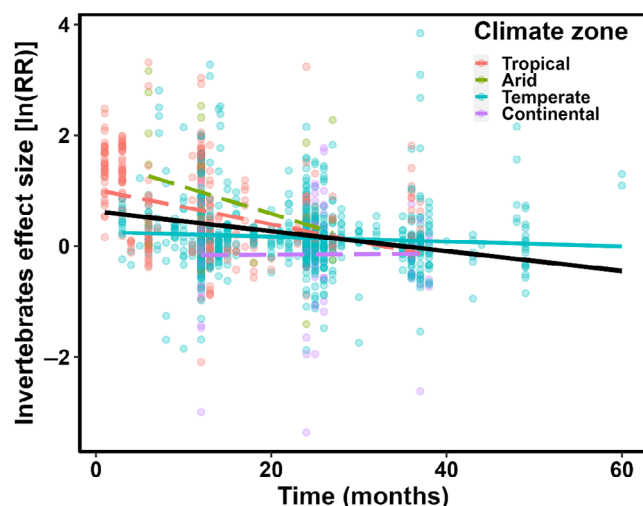
Fig. 5. Effect of incubation duration on invertebrate effect on woody debris (WD) decomposition across climatic zones. Values above versus below zero indicate an increase versus decrease, respectively, in WD decomposition by invertebrates. Climate zones are based on Köppen Geiger climate classifications. This classification recognises five main zones: tropical, arid, temperate, continental and tundra. The continental zone includes the boreal climate zones. Dashed lines are not significant, solid lines are statistically significant. The black line represents the overall trend regardless of climate zone.
