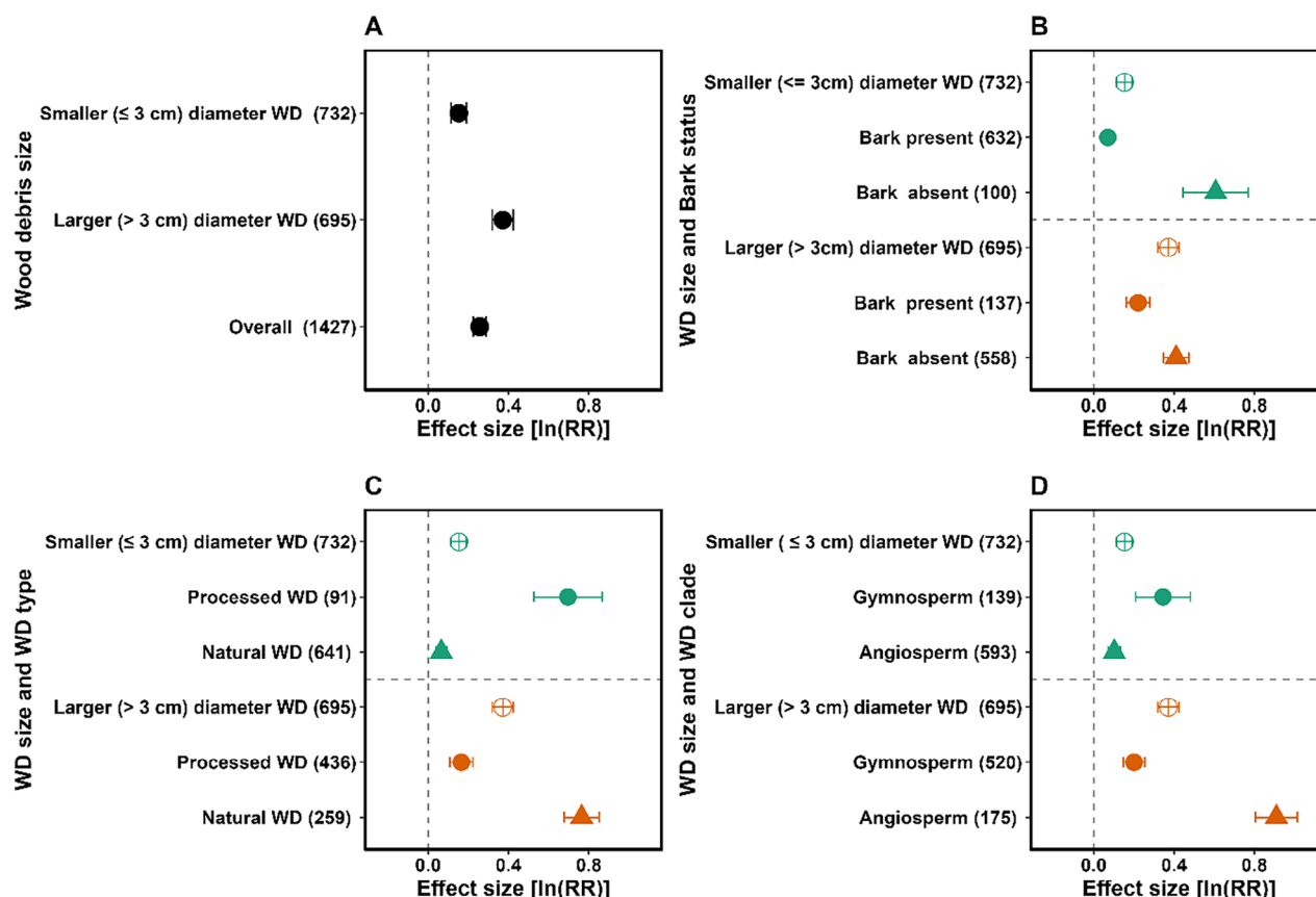
Fig. 3. Effect of woody debris (WD) diameter on the invertebrate contribution to WD decomposition (A) and its effect under different bark status (B), WD type (C), and WD clade (D). Effect sizes with error bars crossing zero (vertical dashed line) are not significantly different from zero. Numbers in parentheses are the number of observations. The WD diameter range for ‘smaller’ WD was 0.3–3 cm and the range for ‘larger’ WD was 3.1–23.1 cm.
