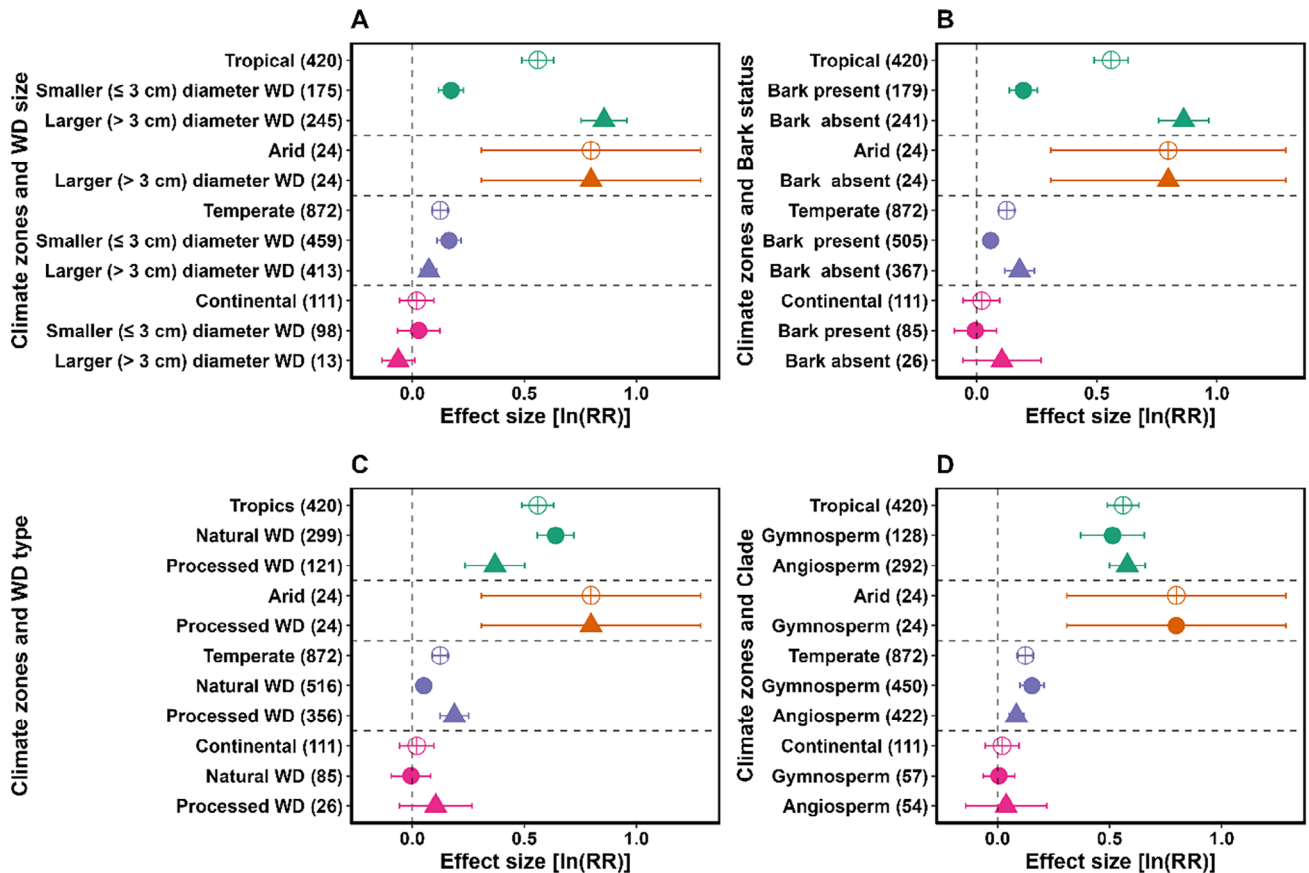
Fig. 4. Effects of woody debris (WD) diameter (A), bark status (B), WD type (C), and WD clade (D) on the invertebrate contribution to WD decomposition across climate zones. The climate zones were classified based on Köppen Geiger climate classification. Effect sizes with the error bars crossing zero (vertical dashed line) are not significantly different from zero. Numbers in parentheses are the number of observations.
