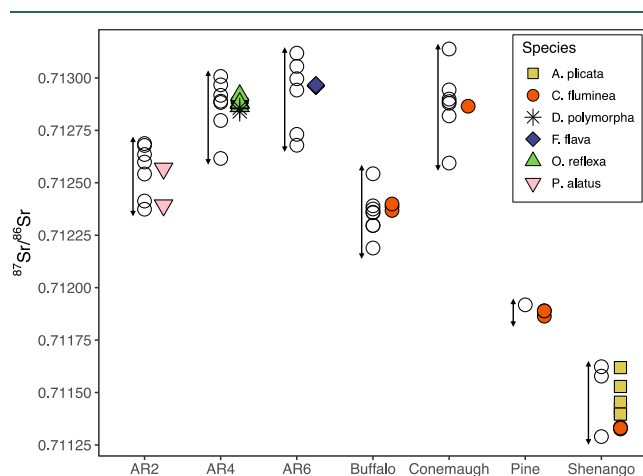
Figure 3. Sr isotope ratios for each sample collected, with stream samples (open circles) plotted with corresponding shells. ^{87}\text{Sr}/^{86}\text{Sr} values for all shell samples fall within the range of ^{87}\text{Sr}/^{86}\text{Sr} values for streamwater from which it was collected. Analytical error for each sample is smaller than symbol. AR = Allegheny River, with numbers corresponding to navigation pool.
