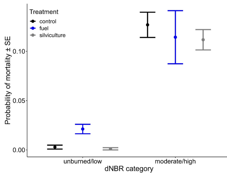
Fig. 3 Probability plus/minus standard error of tree mortality for mature trees within three months following the Frye Fire (2017) in the Pinaleno Mountains in southeastern Arizona, USA. Mortality was calculated using a combination of lidar and remotely sensed satellite imagery
