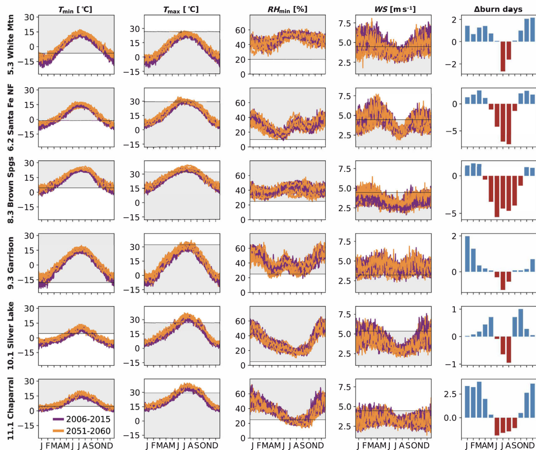
Fig. 4 | Annual variability of climate constraints for RCP4.5 CMIP5 simulations. Data from 18 models is shown, with each line representing one model. Columns represent T_{\min} , T_{\max} , RH_{\min} , and WS (purple: 2006–2015, orange: 2051–2060), as well as model-average change in burn days between present day and future climate
