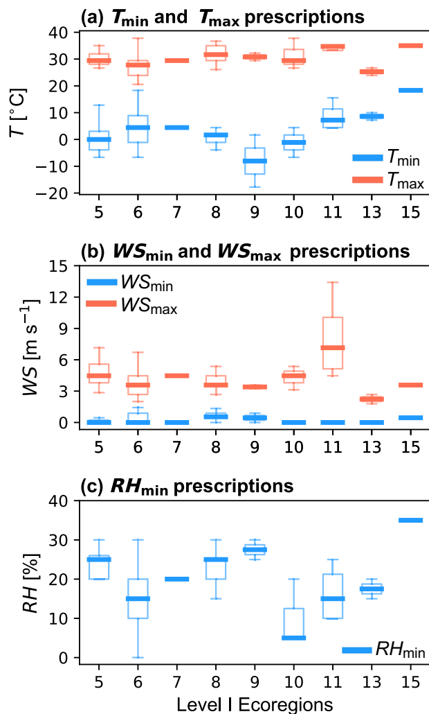
Fig. 7 | Ranges of prescriptions grouped by EPA Level I ecoregion. a minimum and maximum temperature, b minimum and maximum wind speed, and c minimum relative humidity. Prescription ranges highlight strong variability across as well as within ecoregions. The box-plot center lines represent the median of all prescriptions within the Level 1 ecoregion, the box limits represent the upper and lower quartiles, and the whiskers extend from the box to the farthest data point lying within 1.5x the interquartile range from the box.
