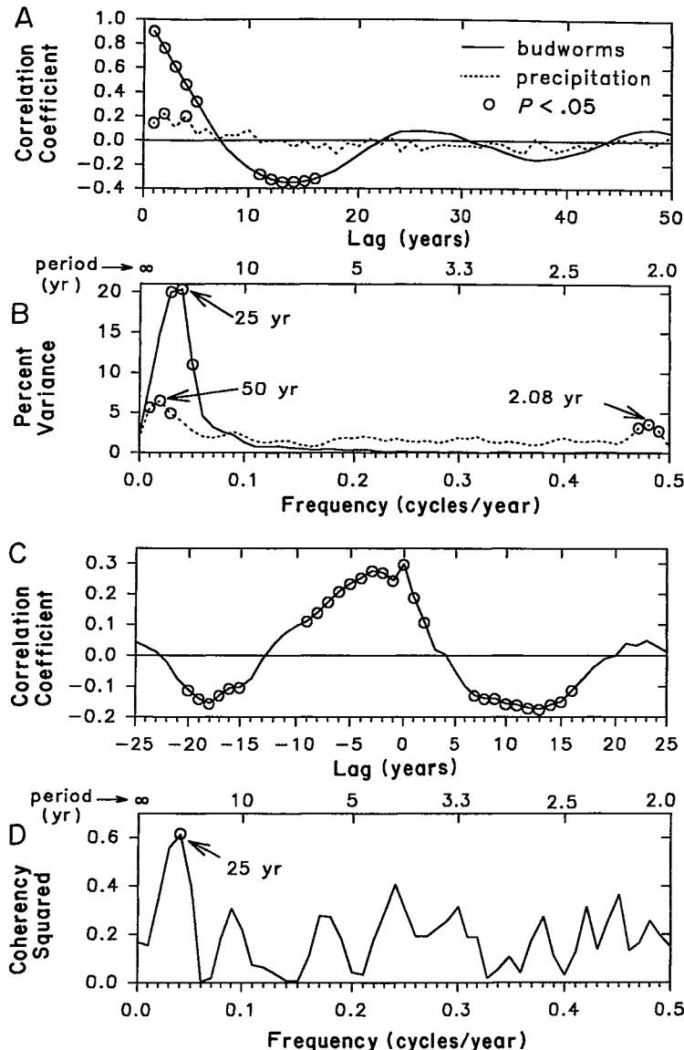
FIG. 11. (A) Autocorrelation functions of reconstructed regional budworm time series and spring precipitation (1600–1989), (B) univariate power spectra of the two time series, (C) cross-correlation function of budworms and precipitation, and (D) coherency squared spectra from the bivariate spectral analysis of budworms and precipitation. Circled values were significant at P < .05 .
