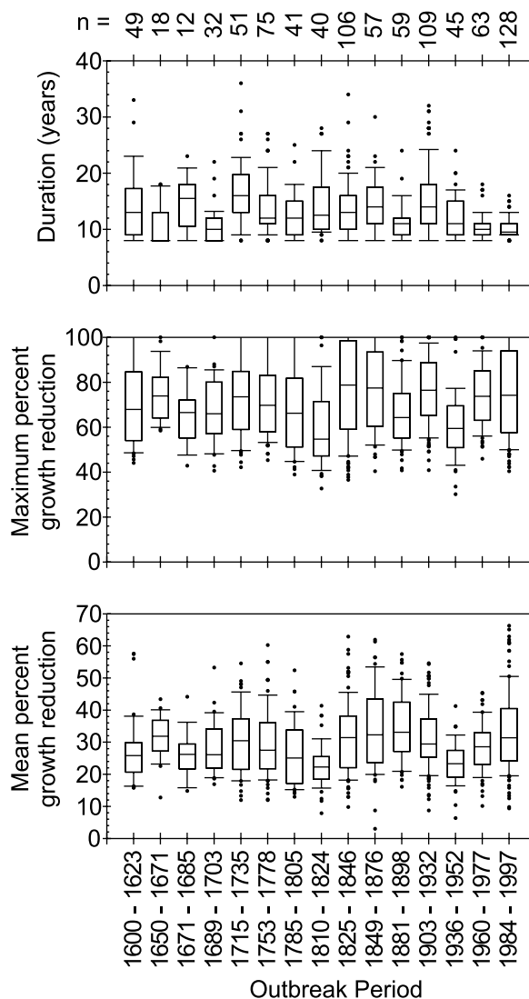
Fig. 7. Box plots of the characteristics of reduced growth periods in individual Douglas-fir trees. Trees were grouped into periods of increased activity over the entire Rio Grande National Forest. Trees were included only if at least 50% of the trees at the individual site exhibited growth reductions that met the outbreak criteria. The number of trees meeting this criteria is shown at the top. The boxes represent the 25th, 50th, and 75th percentiles, while the tails represent the 10th and 90th percentiles.
