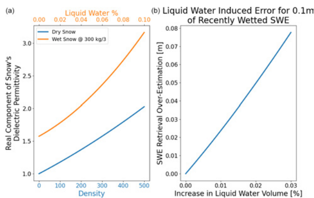
Figure 8. (a) The theoretical dielectric permittivity for varying snow density (blue) and wetness (orange, constant 300 \text{ kg m}^{-3} density) using the equations from Tiuri et al. (1984). (b) SWE retrieval errors caused by 0.1 \text{ m} of SWE that increased by varying liquid water percentages in wetness between SAR images.
