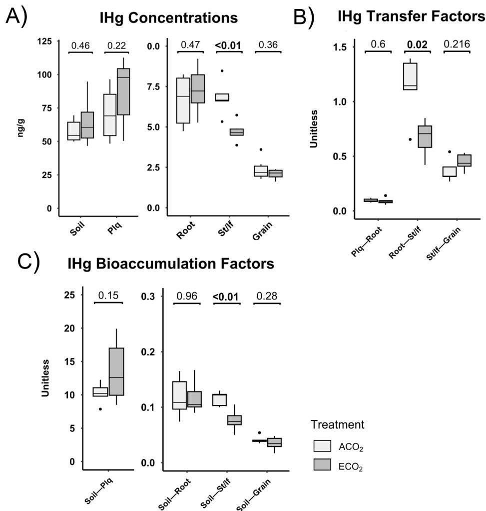
Fig. 3. IHg concentrations, bioaccumulation factors, and transfer factors in the soil-plant-grain system. All graphs compare the \text{ECO}_2 and \text{ACO}_2 treatments. (A) IHg concentrations; from left to right, paired boxplots comparing IHg concentrations in soil, iron plaque, roots, stem/leaf (st/lf), and grain. (B) IHg transfer factors between each compartment and the soil with the source compartment listed first and the sink compartment listed second along the x-axis. (C) IHg bioaccumulation factors within the plant with the source (soil) listed first and the sink listed second along the x-axis.
