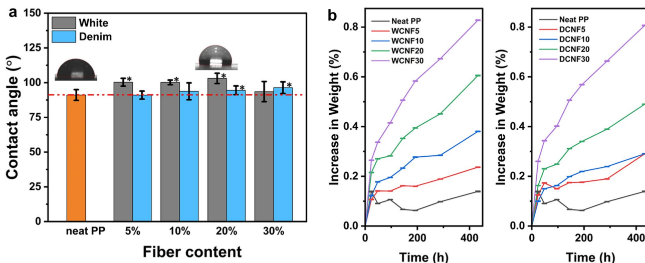
Figure 7. Surface contact angles (a) and water uptake (b) of neat PP and ASA-SMC-cotton/PP composite. The star indicates the difference with neat PP was significant ( p < 0.05 ) using Student's t -test.
