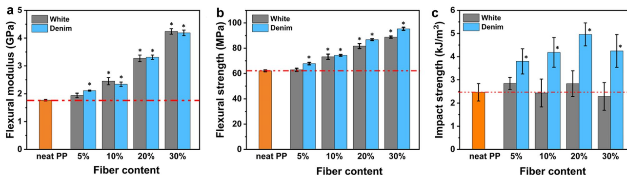
Figure 5. Graphs for the (a) flexural modulus, (b) flexural strength, and (c) impact strength of neat PP and ASA-SMC-cotton/PP composites with different fiber loadings. The star indicates the difference with neat PP was significant ( p < 0.05 ) using Student's t-test.
