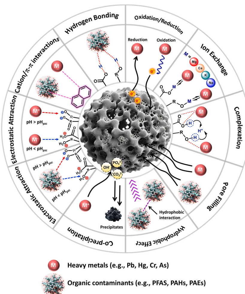
Fig. 4. Interaction mechanism between heavy metals and organic pollutants with biochar particles.
