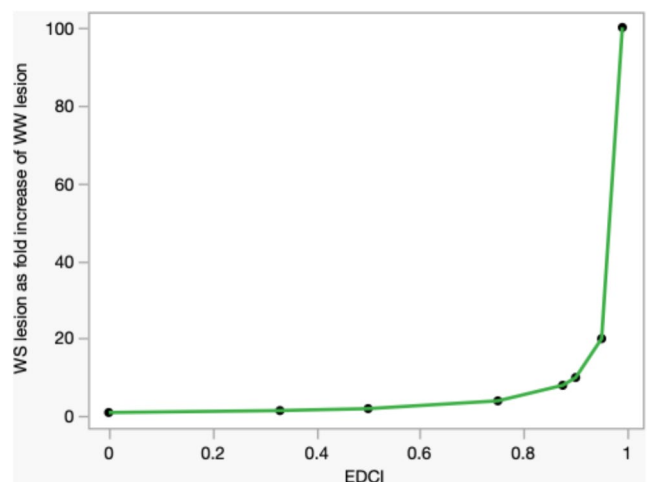
Fig. 4 Positive values of the Environmental Disease Component Index (EDCI) on the x axis and the increase in disease symptom severity associated with the presence of an environmental stressor (water-stressed or WS lesion) on the y axis, expressed as fold-increase (1x, 2x, 10x, etc.) of the disease symptom severity measured in the absence of the stressor (well-watered WW lesion). Note that the EDCI is asymptotic as it approaches its maximum positive value of 1. If disease symptoms severity decreases in the presence of a stressor, the EDCI will be negative
