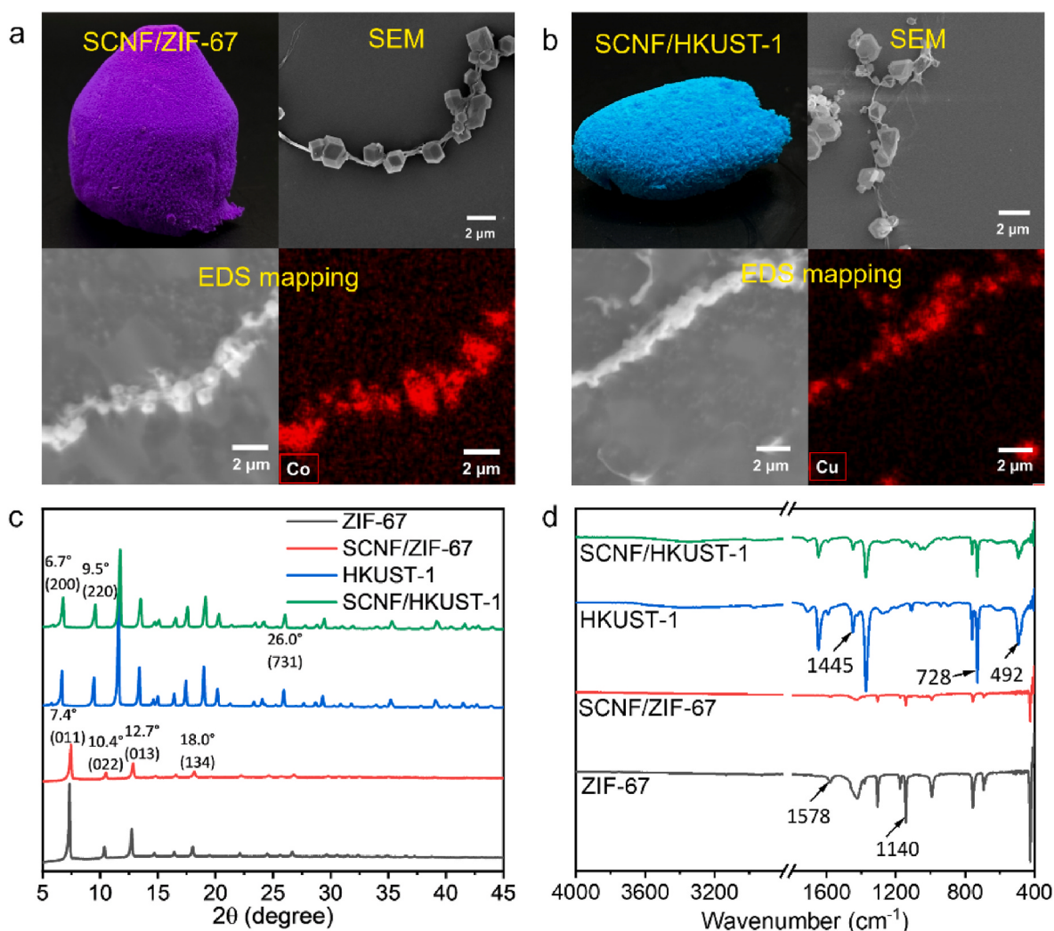
Fig. 5. Characterization of SCNF/ZIF-67 and SCNF/HKUST-1: visual appearance, SEM images, and EDS mappings of SCNF/ZIF-67 (a) and SCNF/HKUST-1 (b), XRD patterns (c), and FTIR spectra (d).
