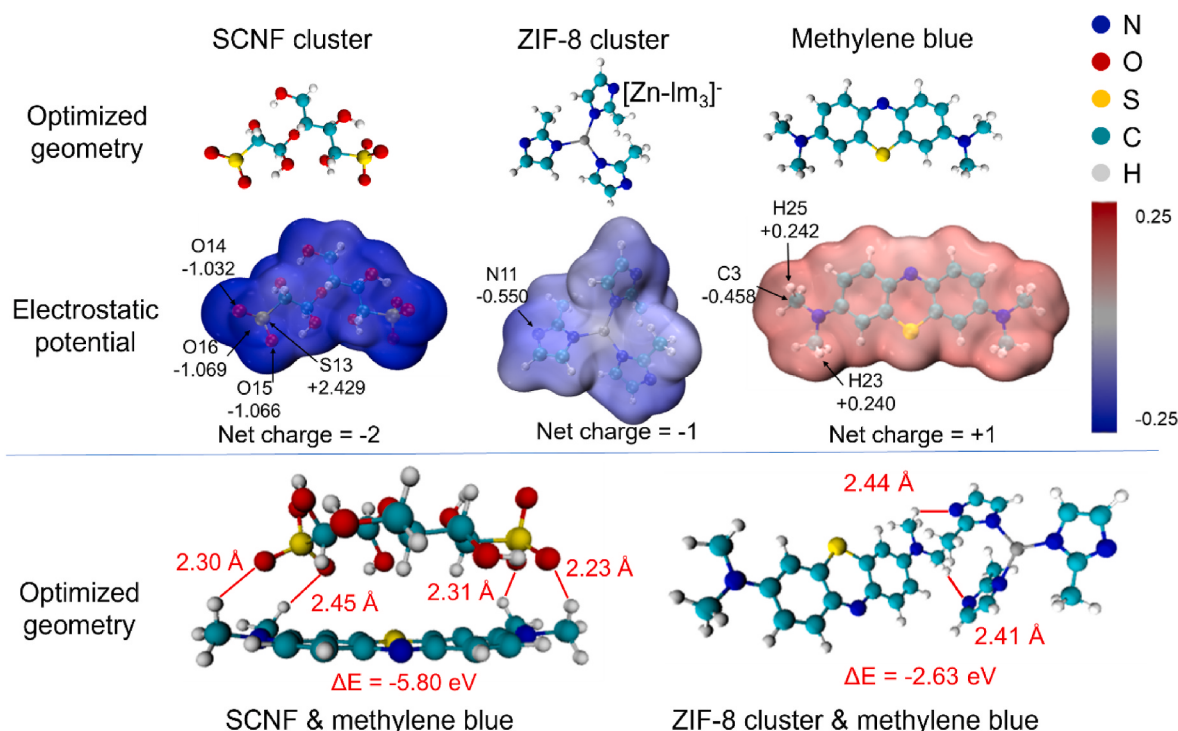
Fig. 7. Optimized geometries and electrostatic potential mappings of SCNF cluster, ZIF-8 cluster, and methylene blue, and optimized geometries of the complexes.
