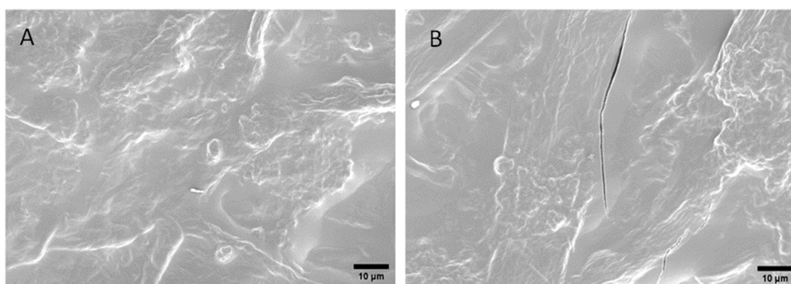
Figure 12. Electron micrograph of TOCN-coated paper surface without sonication (A) and with 10 kJ/g of sonication (B). Scale bars represent 10 \mu\text{m} .
