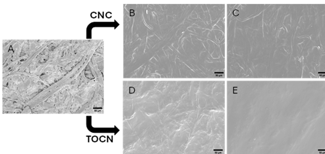
Figure 1. SEM micrographs of uncoated copy paper, and CNC- and TOCN-coated paper surfaces; (A) uncoated copy paper; (B,C) CNC coatings with doctor blade settings of 50 and 100 µm, respectively; (D,E) TOCN coatings with doctor blade settings of 150 and 2000 µm, respectively. Scale bars represent 50 µm.
