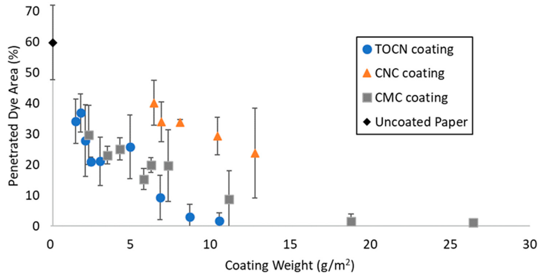
Figure 6. Grease penetration for creased paper samples. Coating speed was approximately 11 mm/s.
