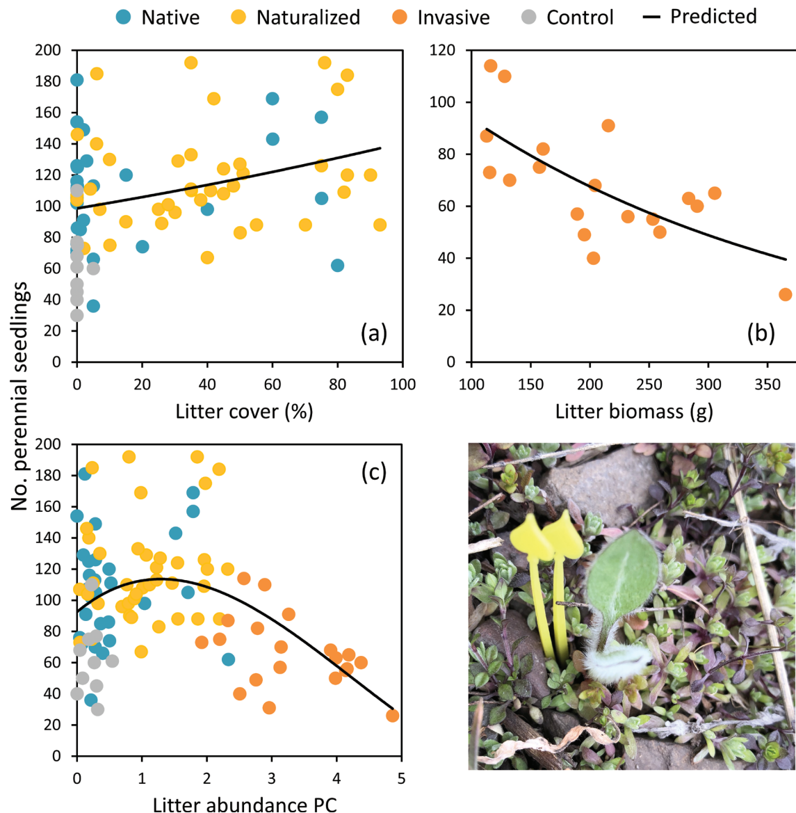
Figure 5. Relationships between recruitment of perennial seedlings in 2018 and litter abundance. Litter abundance was measured by a litter cover for treatments representing native or naturalized annuals and controls, b litter biomass for the invasive annual treatment, and c a principal component combining both litter metrics to visualize the unimodal relationship across all treatments (this relationship was also significant when we ran a parallel model using 2017 data: F_{1,97} = 17.5 , P < 0.001 ). Photo shows a perennial forb ( Balsamorhiza sagittata ) seedling emerging amidst sparse litter in a naturalized plot. Note that recruitment was modeled with a negative binomial distribution in all cases and associated predicted relationships have been back-transformed to the original scale.
