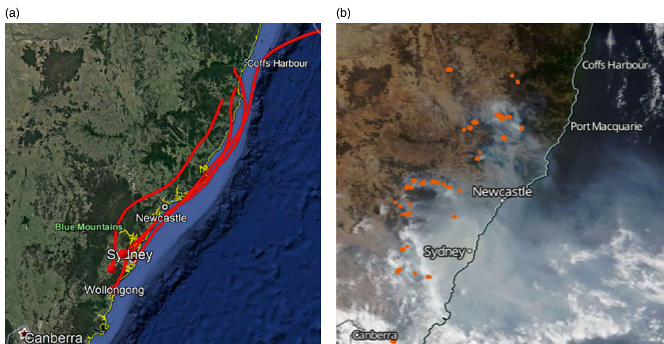
Figure 9.7 (a) HYSPPLIT in NSW 24 hr back-trajectories starting at 1000 29 December 2019 from locations in Sydney and Wollongong; (b) Terra/MODIS satellite imagery on the same day showing hot spots (fires) and smoke plumes on the northern coast and in eastern New South Wales.
