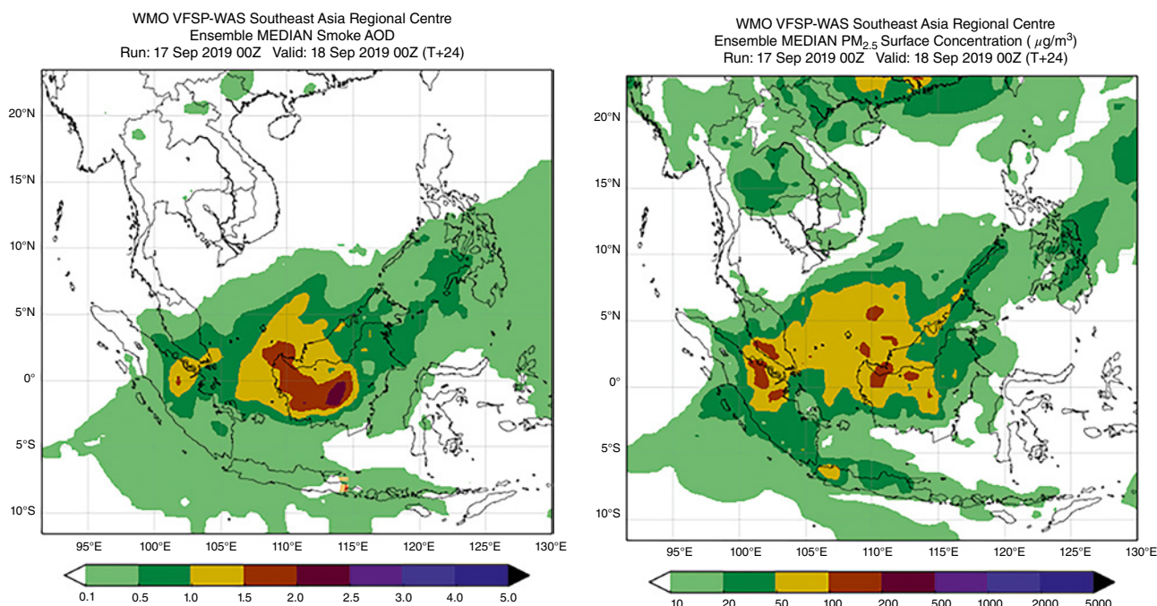
Figure 9.11 Example of Southeast Asia VFSP-WAC multimodel ensemble median 1 day forecast of smoke AOD (left) and PM_{2.5} surface concentration (right) for Southeast Asia in September 2019.
