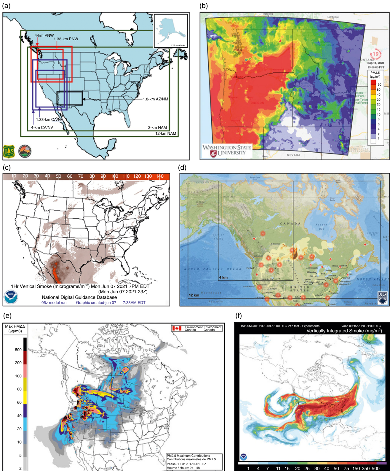
Figure 9.3 Domains of the north American smoke and air quality prediction systems summarized in this section. (a) U.S. BlueSky smoke modeling framework and smoke prediction system, (b) Air Indicator Report for Public Access and Community Tracking (AIRPACT) system, (c) U.S. National Air Quality Forecast Capability (NAQFC) system, (d) BlueSky Canada smoke forecasting system and Canadian wildland fire information system, (e) FireWork Canada, (f) U.S. NOAA operational Rapid Refresh-Smoke (RAP-Smoke) system, (g) High-Resolution Rapid Refresh-Smoke (HRRR-Smoke) System, (h) southeastern U.S. RiRes system.
