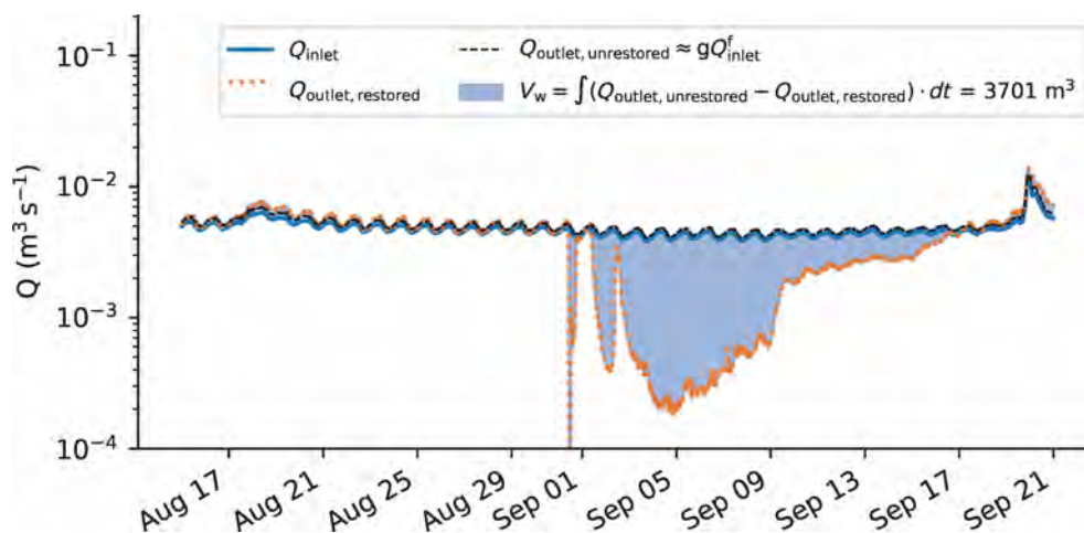
FIGURE 5 | Discharge during the restoration period, which began 30 August 2022. The black dashed line plots the outlet discharge ( Q_{\text{outlet,unrestored}} ) predicted from the power-law equation derived during the pre-restoration period, and represents the counterfactual discharge that would have occurred without restoration. The inlet gage discharge (blue trace) was unaffected by restoration activities, whereas the actual outlet gage discharge ( Q_{\text{outlet,restored}} ; orange trace) dropped significantly below the counterfactual discharge during and immediately after restoration. The integrated difference between the Q_{\text{outlet,unrestored}} curve and the Q_{\text{outlet,restored}} (blue shading) provided an estimate for the increase in meadow water storage due to restoration.
