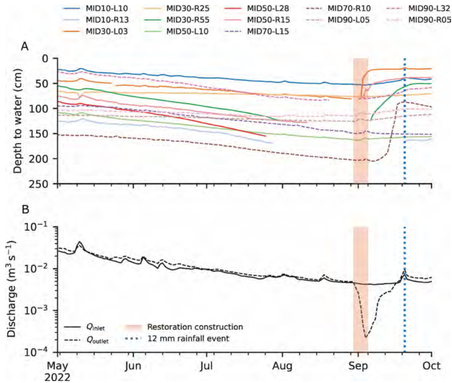
FIGURE 4 | Groundwater depths (A) and streamflow for the upper ( Q_{inlet} ) and lower ( Q_{outlet} ) gaging stations (B) before, during (red shading) and after restoration. Groundwater wells in (A) are plotted with dashed lines for Reach 1 and solid lines for Reach 2. Groundwater data gaps occurred when water levels dropped below the pressure transducer. Well labels describe their position, with the first two numbers representing the transect (10%, 30%, 50%, 70% or 90% of meadow area), the L or R indicating to the left or right of the channel looking downstream, and the last two digits representing the distance from the left or right bank in metres (e.g., MID10-L10 is on the 10% transect, 10m from the stream's left bank). Transects 10, 30, and 50 were in Reach 1, and transects 70 and 90 were in Reach 2.
