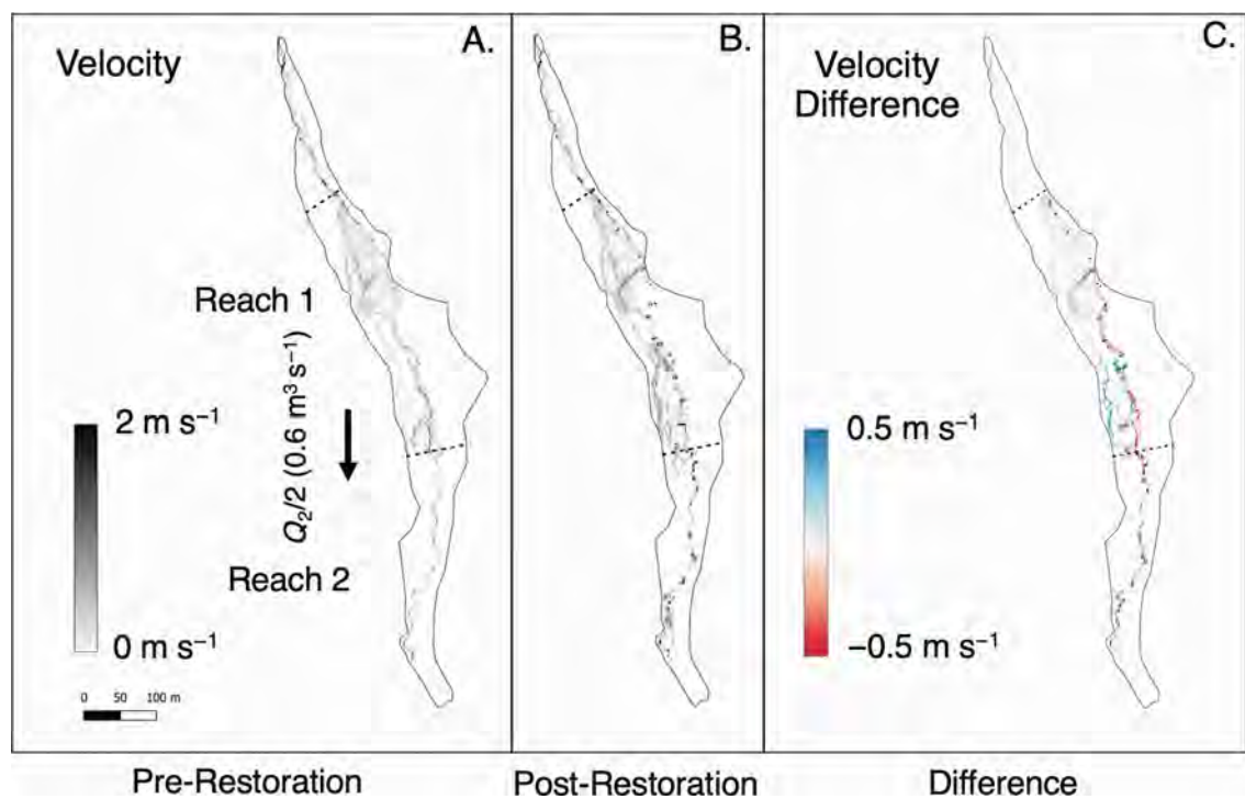
FIGURE 8 | Predicted velocities for Q_2/2 ( 0.6 \text{ m}^3 \text{ s}^{-1} ) for (A) the pre-restoration scenario, (B) the post-restoration scenario using the same scale bar as (A), and (C) the difference in velocity between the restored scenario and the pre-restoration scenario. Dashed black lines indicate the upstream extent of each reach and black outlines show locations of restoration structures.
