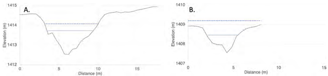
FIGURE 9 | Predicted water surface elevations for Q_2/2 ( 0.6 \text{ m}^3 \text{ s}^{-1} ) for the pre-restoration scenario (solid light blue line) and the post-restoration scenario (dashed dark blue line) using the modified DEM (dashed black line) as input topography for (A) cross section 70 and (B) cross section 90, both located in Reach 2. The modified DEM includes dry and submerged surface elevations.
