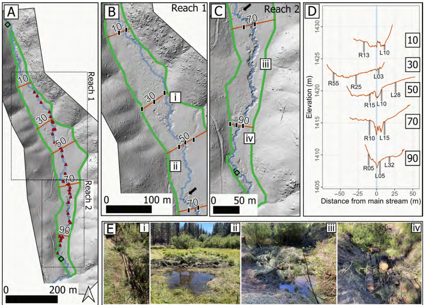
FIGURE 2 | (A) LiDAR-derived hillshade showing Middle Creek Meadow outlined in green and Middle Creek shown in blue. The boxes show Reach 1 (490 m) and Reach 2 (420 m), groundwater transects (orange lines) labelled with the percent upstream meadow area, gaging stations designated by black diamonds, and 35 of 39 restoration structures installed in August 2022 as maroon triangles. Detailed view of (B) Reach 1 and (C) Reach 2. Vertical black bars indicate groundwater well locations. The black arrow indicates the location of the headcut separating Reach 1 and Reach 2. (D) Cross-section elevation profiles for Middle Creek at each transect. Lines are centred on the thalweg of the main channel prior to restoration. Grey bars indicate groundwater well locations and depths. (E) Photos showing restoration structures. Locations of photos are shown with corresponding Roman numerals in (B) and (C). From upstream (Reach 1) to downstream (Reach 2): (i) 8 conifers packed into substantial meadow headcut, (ii) 11 m wide channel-spanning structure, (iii) downed conifers placed into 1.3 m deep incised channel, and (iv) conifers placed into incised meadow channel.
