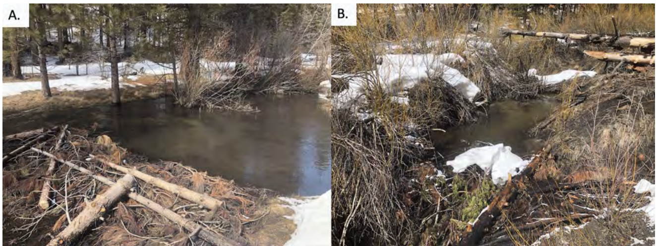
FIGURE 7 | (A) Beaver dam analog (BDA) in Reach 1 with the top of the dam at the same elevation as the top of channel banks. (B) A BDA in Reach 2 with the top of the dam below incised channel banks. Both structures captured sediment following the first winter post-restoration. Photo credit: Patrick Jarrett, California Department of Water Resources.
