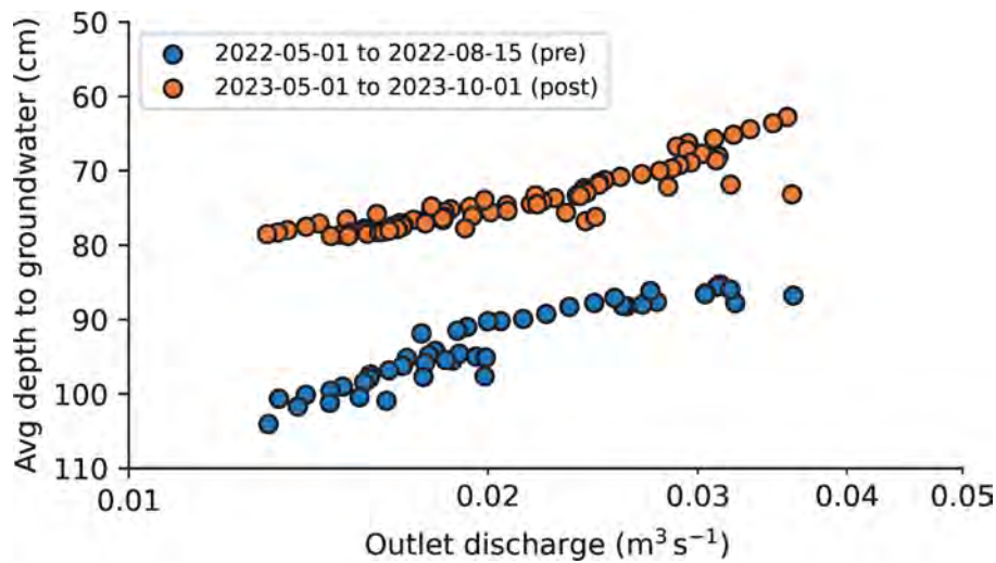
FIGURE 6 | Average depth to groundwater across all instrumented meadow wells before (blue) and after restoration (orange) as a function of shared outlet discharge (log scale). The 2023-shared discharge values were later in the summer because of the wetter winter and longer recession limb and possibly the influence of the higher groundwater elevations on baseflow.
