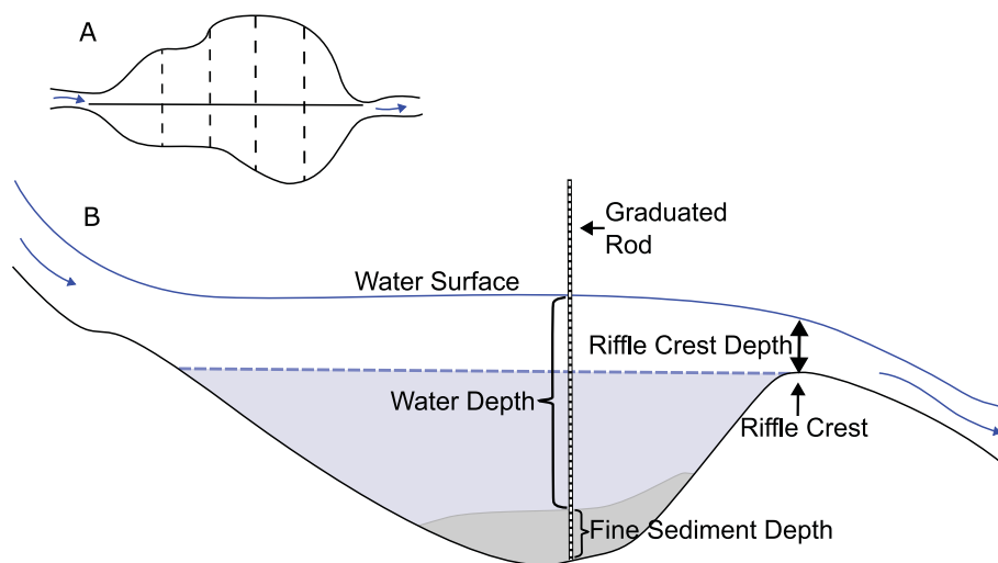
FIGURE 3 | The volume of residual sediment and water in pools was estimated using the V^* method described by Lisle and Hilton (1992). The length and distance between 3–7 equally spaced cross sections in each pool were measured to estimate pool area (A). Total water depth and depth of fine sediment were measured along the pool cross sections at ~20 equally spaced points, and riffle crest depth was subtracted from pool depth measurements to estimate the residual pool volume (B). Figure modified from Lisle and Hilton (1992).
