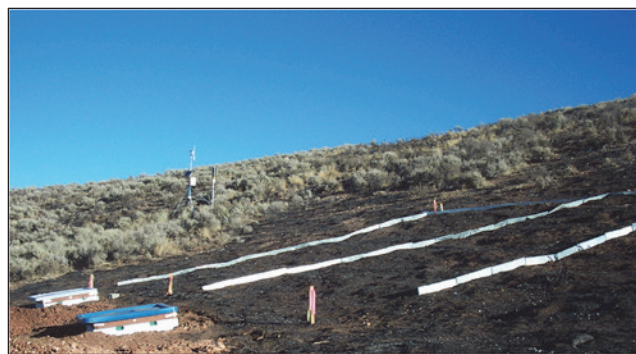
Figure 5. Installation of the plot borders on two of the burned plots on Burn Unit 11 in October 2003. On the lower left are the covers over the boxes containing the sediment basins and tipping bucket devices (fig. 7). The bottom gutters to divert runoff and sediment from the bordered plots to the sediment basins (fig. 6) have not yet been installed. The weather station is in the background still on Burn Unit 11, but the burn was less severe on the Red Mountain Burn Erosion study (photo by I. S. Miller).
