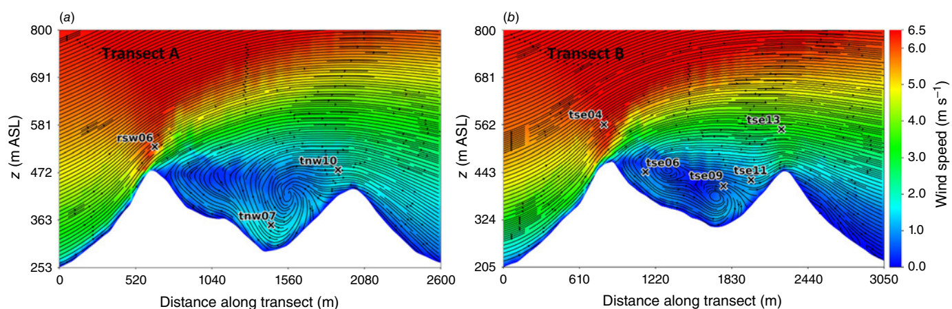
Fig. A24. Side view of the modelled flow field through (a) Transect A, and (b) Transect B for the Base Case ( k -epsilon model). Tower labels indicate maximum sensor height for that tower.
