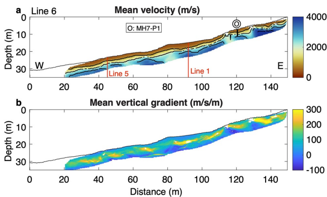
Figure 5. Results of Line 6 inversion. (a) Interpolated mean velocity model with contour lines at 1,000, 2,000, 3,000, and 4,000 m/s. The model is masked out below the deepest raypath and where CoV >40%. Black dashed lines highlight the locations of boreholes within 10 m of the survey line. Red lines indicate the intersection points with Line 5 (45 m) and Line 1 (90 m). (b) Mean vertical velocity gradient (m/s/m).
