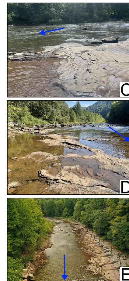
Figure 2. (A–B) Uncrewed aerial vehicle photogrammetry-derived orthomosaics (2 cm resolution) showing aerial views of data collection locations. Blue arrows show flow direction. (A) Price Formation sandstone (SS) bedrock reach, with the finer sandstone upstream (right side of the image) and coarser sandstone downstream (left side). (B) Greenbrier Group carbonate bedrock reach. (C–E) Site photographs for the fine sandstone, coarse sandstone, and carbonate reaches, respectively. Locations of photos are marked on A and B. Note that the foregrounds of C and D are ~2 m across the photo, while that of E is ~35 m across. The visually prominent fractures in the carbonate reach are widely spaced relative to fractures in the sandstone reaches (see Results section); sandstone reaches display missing centimeter-scale blocks of rock along bedding and fracture planes (foreground of C and D).
