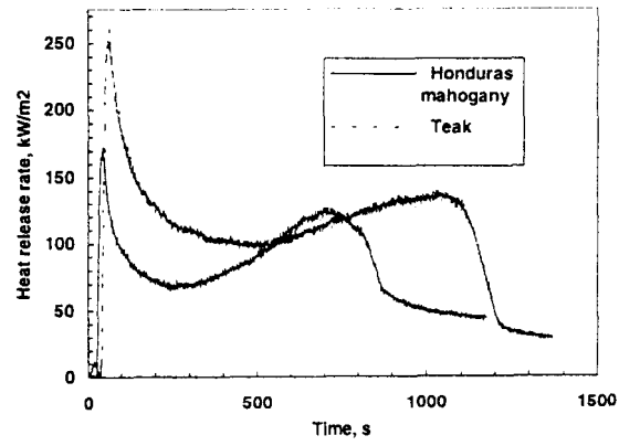
Figure 2. Rate of heat release rate curves for Honduras mahogany and teak.
