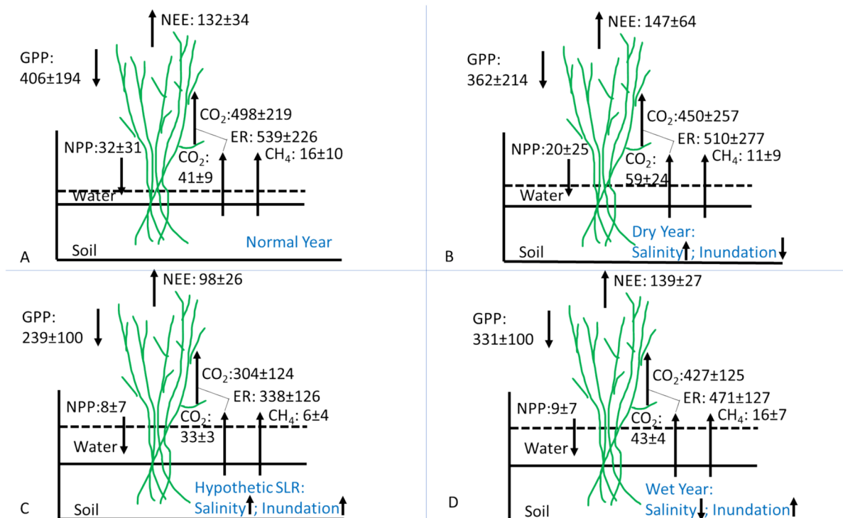
Fig. 8 Diagram showing the averaged carbon fluxes (unit: \text{g C m}^{-2} \text{ yr}^{-1} ) under the normal, dry, wet years, and hypothetical SLR in the brackish marsh sites in Terrebonne Basin, Louisiana using
