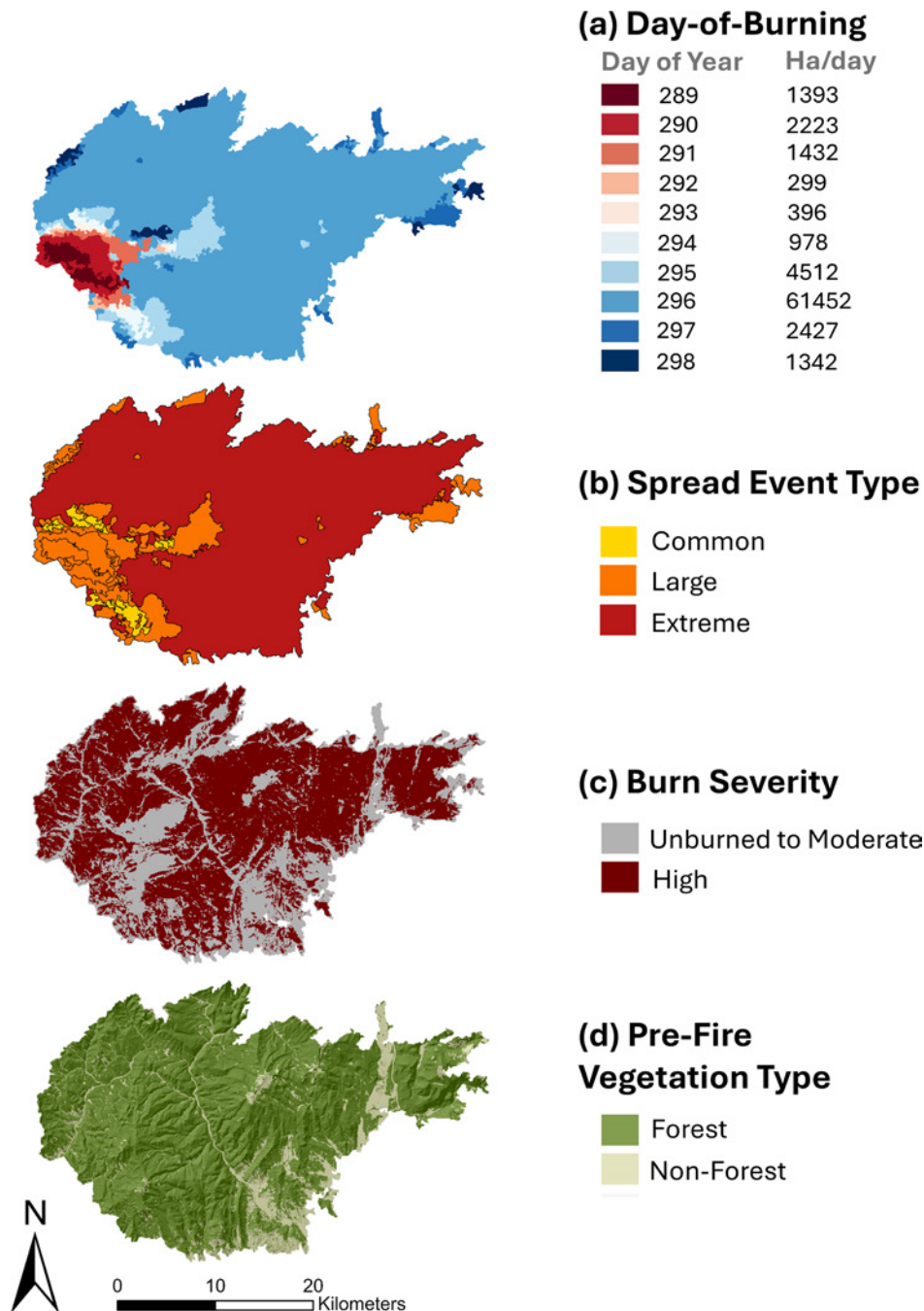
FIGURE 2 | Example shows the East Troublesome fire, depicting (a) daily fire progression, (b) categorical fire spread event types, (c) high-severity burn patches (red), and (d) prefire vegetation with topographic relief. The East Troublesome fire burned 78,000 ha in Colorado in October 2020.
