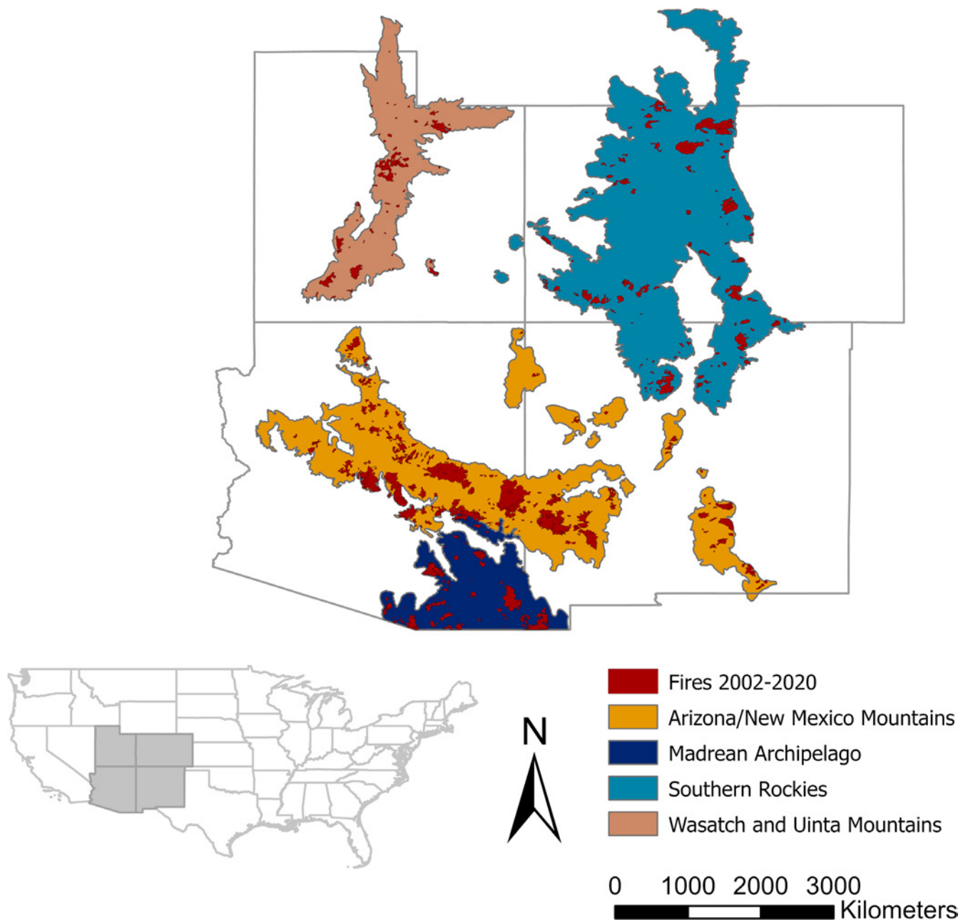
FIGURE 1 | Map of the southwestern US study area, large (>400ha) fire perimeters (2002–2020), and the forested ecoregions included in this analysis (EPA 2023). Map lines delineate study areas and do not necessarily depict accepted national boundaries.
