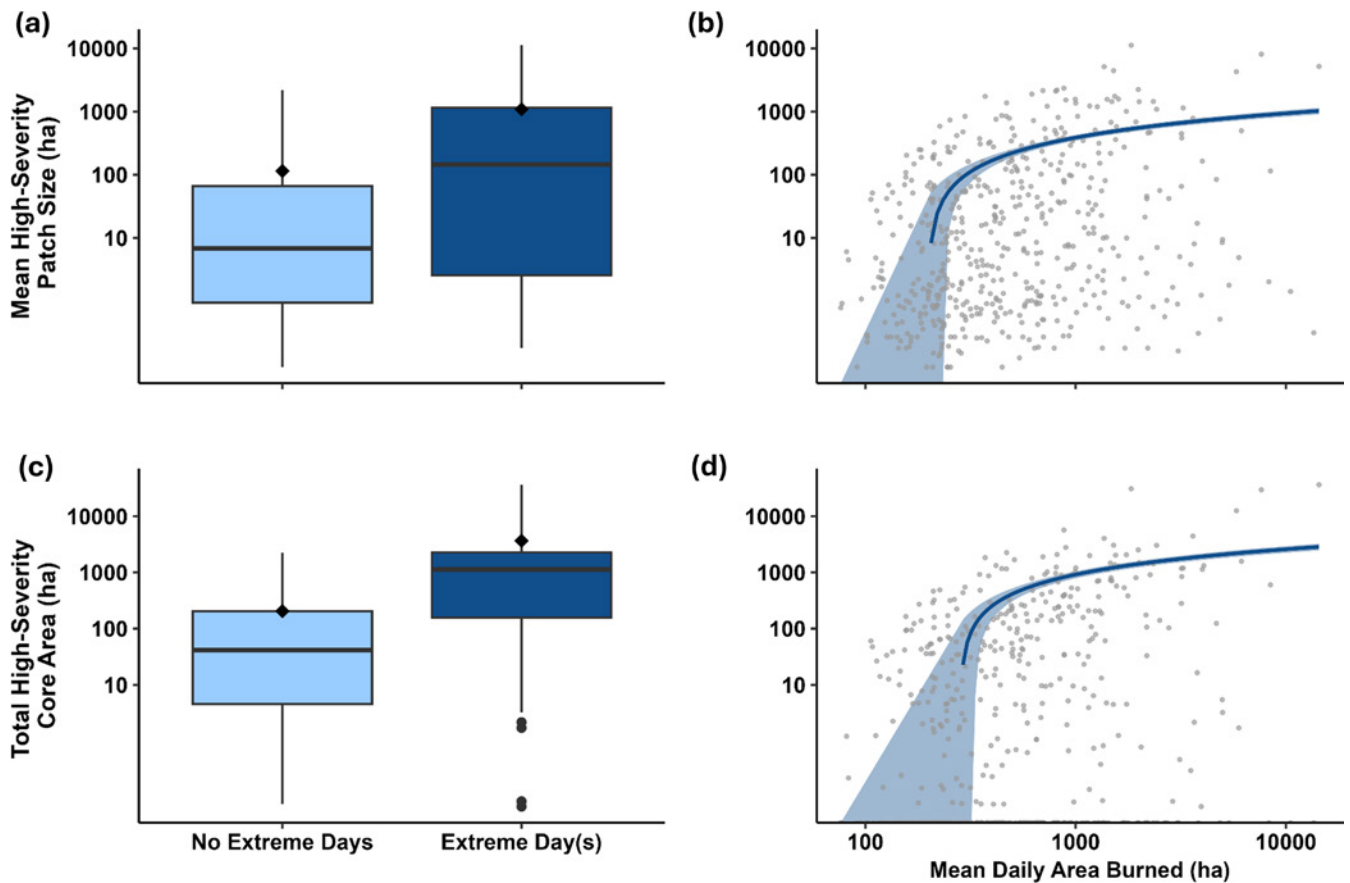
FIGURE 4 | Boxplots and scatterplots showing relationships between fire type, fire spread event size, and landscape metrics of high-severity patches at the fire level. We illustrate relationships between area-weighted mean high-severity patch size (A-B) and total high-severity core area (C-D) with fire spread event types (boxplots in left column) and daily area burned (scatterplots and linear trendlines in right column). Fire type is categorically represented by the boxplots as fires with one or more extreme fire spread events (dark blue; “Extreme Day(s)”) or fires without an extreme fire spread event (light blue; “No Extreme Days”). Central horizontal lines within the boxplots depict median values, black diamonds represent means, and points represent outliers. Geometric means were plotted instead of arithmetic means to account for \log_{10} -transformed Y axes. Scatterplots illustrate metrics plotted against \log_{10} -transformed mean daily area burned (ha). Trendlines on scatterplots include 95% confidence intervals.
