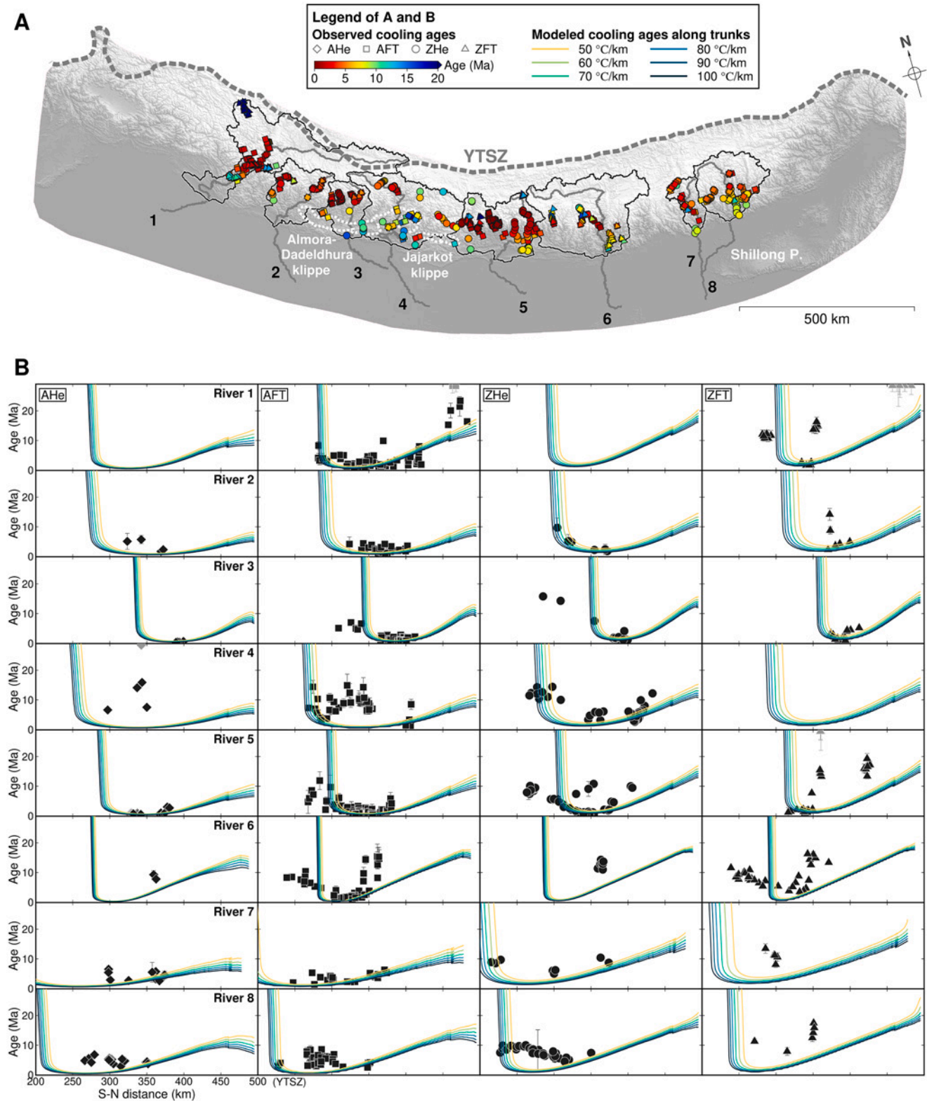
Fig. 5. Comparison of modeled and observed thermochronologic ages. (A) Compilation of thermochronologic ages in the eight Himalayan catchments (van der Beek and Schildgen, 2023). Different thermochronometric systems including Apatite (U-Th)/He (AHe), Apatite fission track (AFT), Zircon (U-Th)/He (ZHe), and Zircon fission track (ZFT) are represented by diamond, square, circle, and triangle, respectively, which are all colored by cooling ages. The eight rivers (gray) with corresponding catchments (black) are shown. (B) Modeled and observed thermochronologic ages for each of the eight catchments, projected on the corresponding black box in Fig. 3A, according to the legend. YTSZ is the north boundary in (A) and (B).
