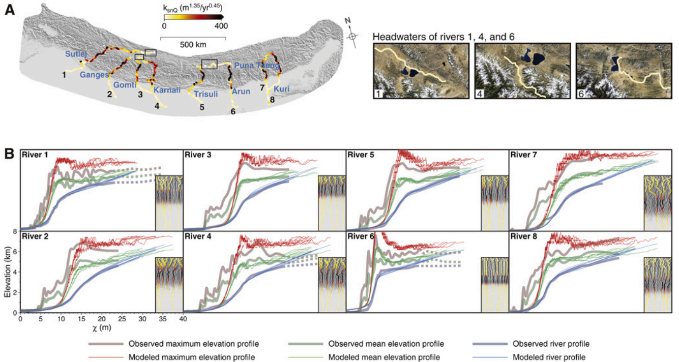
Fig. 2. Comparison of modeled and observed river profiles. (A) Map of the eight of the main Himalayan rivers analyzed, colored by k_{snQ} . The headwaters of rivers 1, 4, and 6 connect with the plateau lakes as shown in Google Earth images, so their upstream parts are in the same elevations in \chi –elevation plots (the dashed lines in (B)). (B) Modeled profiles (thin lines) best fitting the observed profiles (thick lines) for each of the eight rivers (Appendix B). Right-bottom inset on each panel shows modeled topography (the grayed base map) and rivers extracted from 10 headwaters (the lines colored by k_{snQ} ).
