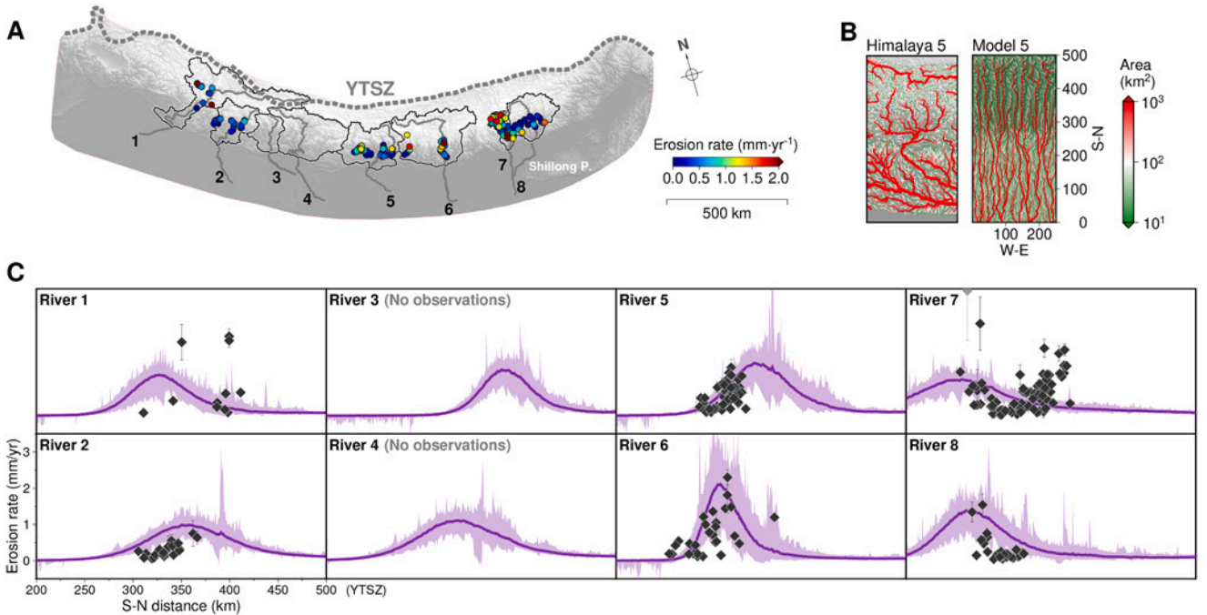
Fig. 4. Comparison of modeled and observed erosion rates. (A) 10 Be-derived tributary-catchment erosion rates in the Himalayas accessed from the Octopus archive (Codilean et al., 2018). The map shows the (trunk) rivers 1–8 (gray thick lines) and corresponding catchments (black thin lines). (B) The stream networks colored by the upstream area in the observed and modeled Himalayas where river 5 drains. (C) Modeled and observed short-term erosion rates for each of the eight catchments, projected on the corresponding black box in Fig. 3A. YTSZ is the north boundary in (A) and (C).
