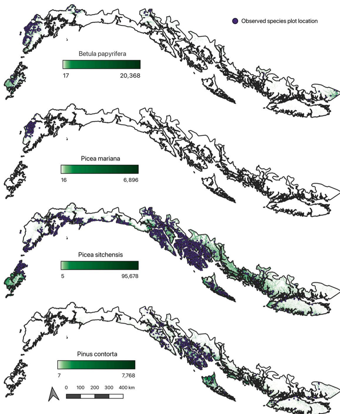
Figure A1B. Mapped results of GNN imputation model for the full modeling region of species biomass (gm -2 ) and extent. The four species select show the spatial constraints around areas of observed presence. Plot locations shown are the publicly available locations from both FIA and FAIB
