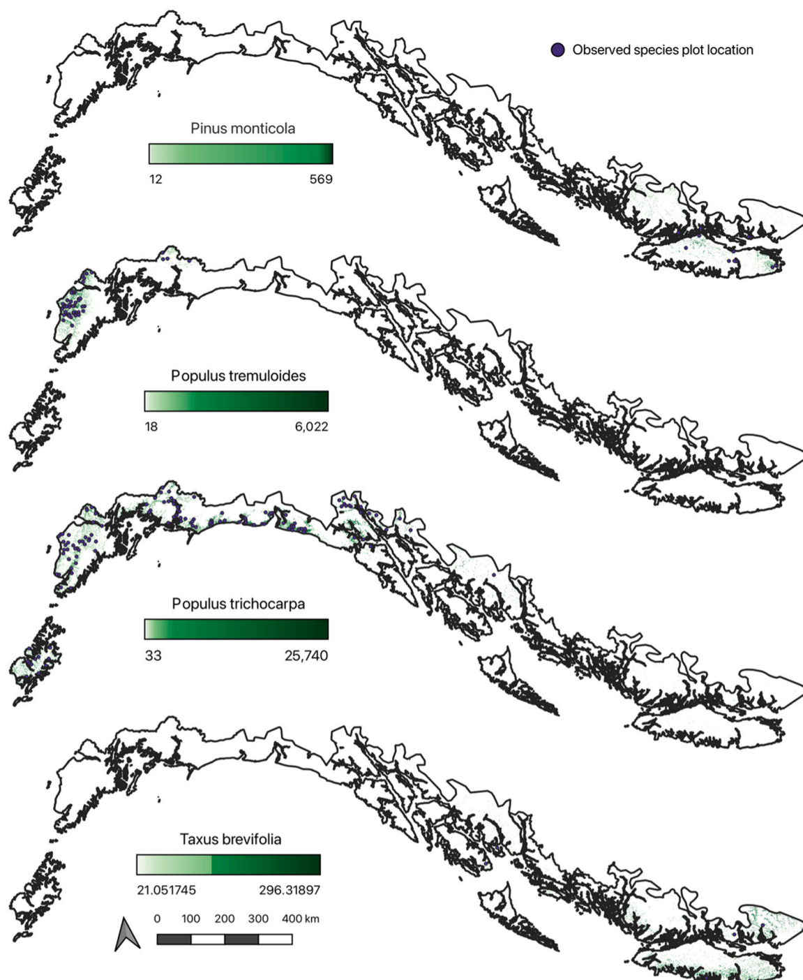
Figure A1C. Mapped results of GNN imputation model for the full modeling region of species biomass (gm -2 ) and extent. The four species select show the spatial constraints around areas of observed presence. Plot locations shown are the publicly available locations from both FIA and FAIB
