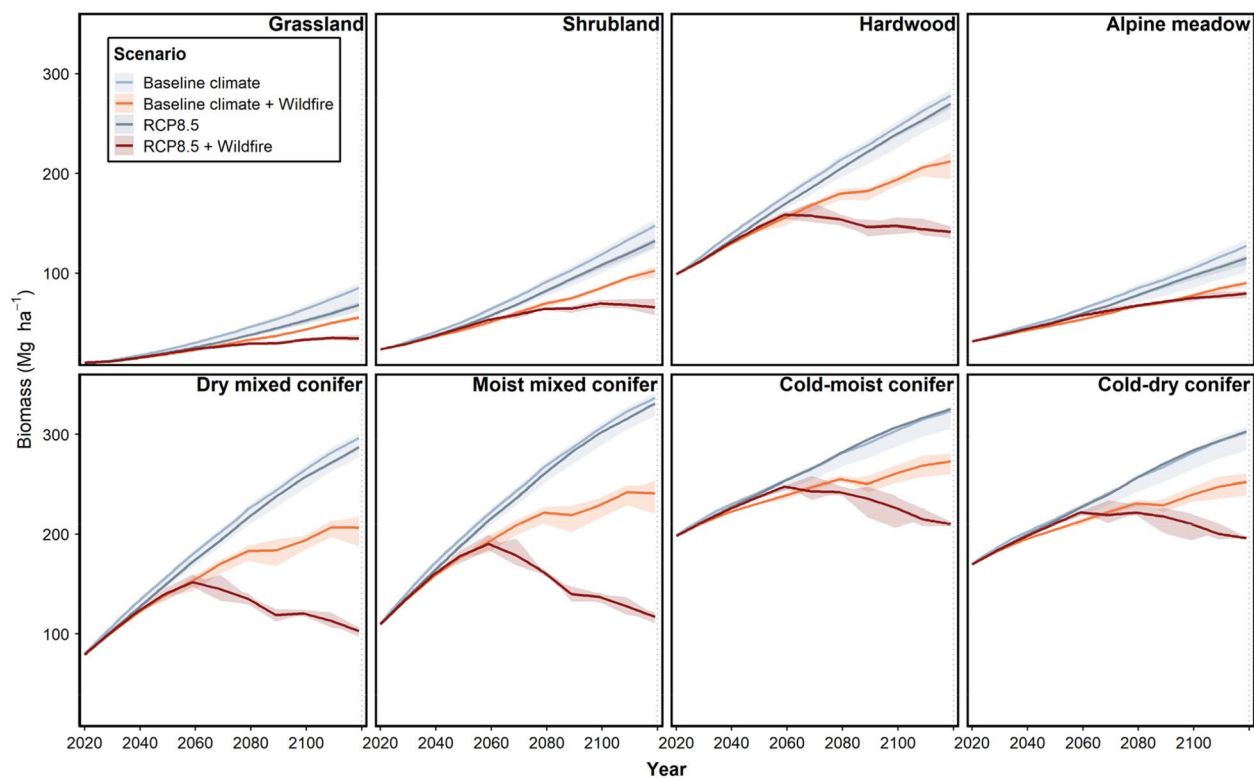
Fig. 2 Biomass accumulation per vegetation type under a No Disturbance scenario (cool colors) and the Wildfire Only scenario (warm colors). Each scenario was run under two climate forecasts: a baseline forecast representing late twentieth century climate ("Baseline climate") and a more realistic forecast based on a RCP8.5 emission scenario ("RCP8.5"). Direct effects of climate change on biomass accumulation were minimal. Wildfire had a substantial impact on biomass under the baseline climate scenario (orange lines), and an even greater impact under the RCP8.5 scenario (red lines)
