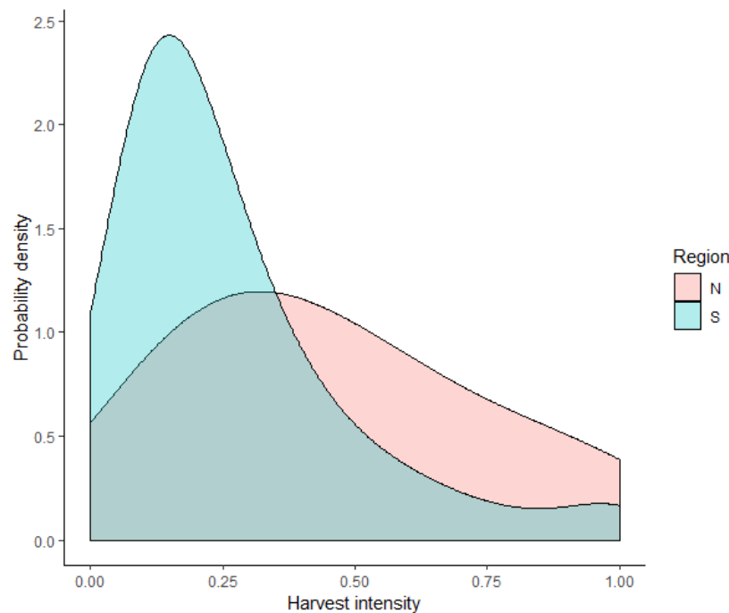
Figure 4. The distribution of harvest intensities for each of the regions (N = Northern Vermont and Northern New Hampshire from the FIA state data, S = all other area in the Connecticut River Watershed states) for one of the 10 replicates. Other replicates had similar distributions.
