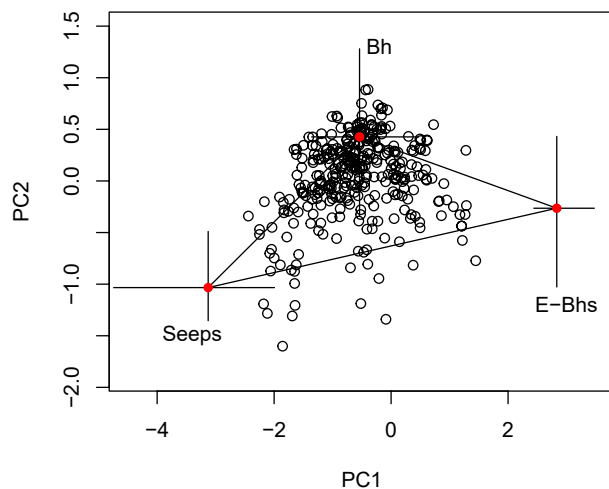
Figure 5. End-member mixing analysis using principal component analysis. The end member mixing model traced the contribution of end member HPUs to stream water during each grab sample. The mixing model used principal components of total Al, Ca, Na, DOC, and pH from seeps, Bh podzols, combined E and Bhs podzols, and streamwater (open circles). The end members show the median principal component values (filled circles) and the inter-quartile ranges as error bars. The medians are connected with lines to show the triangular mixing space for our analysis.
