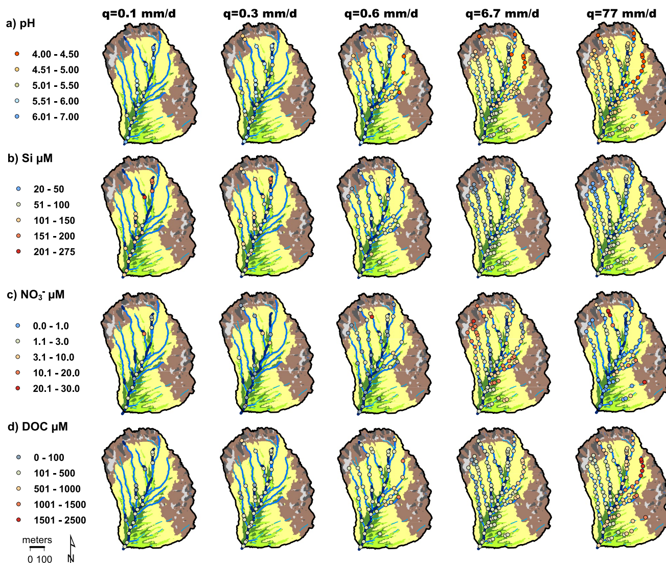
Figure 8. Stream chemistry spatial patterns as stream flow increases. Catchment maps showing how stream chemistry changes as stream flow ( q ) increases and more of the catchment becomes hydrologically connected with the expanding active stream channel and subsurface contributing area. For sampling dates: August 21, 2010; August 6, 2010; July 22, 2015; April 1, 2010; October 1, 2010. Based on data from Bailey and McGuire (2019) for 2010 dates, S. W. Bailey, McGuire, Ross, and Green (2019) for 2015 date. (a) pH; (b) Si; (c) nitrate; (d) DOC. Map colors follow Figure 1: Bedrock histosol (black), E podzol (gray), Bhs podzol (brown), Bimodal podzol (dark green), Bh podzol (light green), perennial stream (heavy royal blue line), intermittent stream (medium blue line), ephemeral stream (fine, light blue line).
