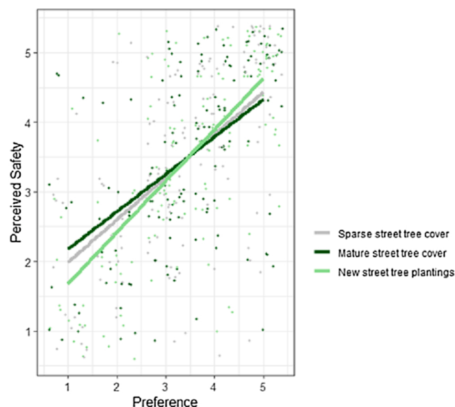
Fig. 4. Two-way repeated measures ANOVA.
