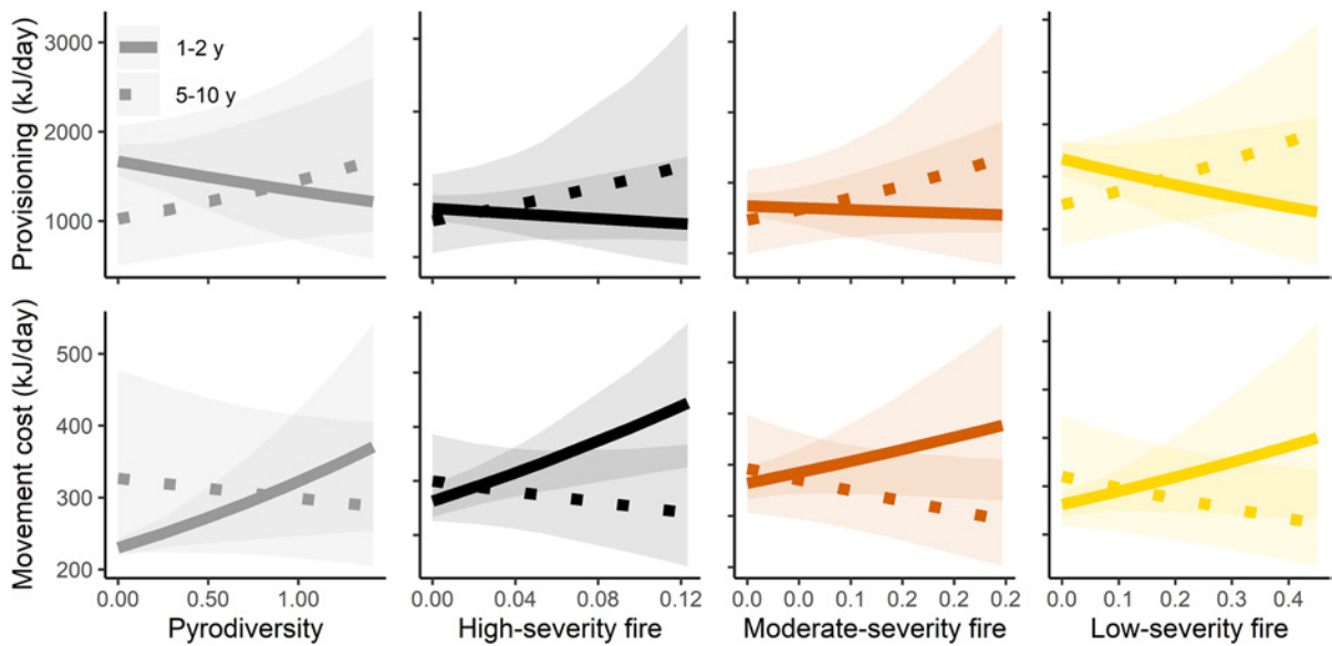
Fig. 5 Predicted effects of fire on provisioning and movement costs. Lines indicate predicted relationships between fire covariates and energetic metrics, and shaded areas indicate predicted 95% confidence intervals. Solid lines show predicted
