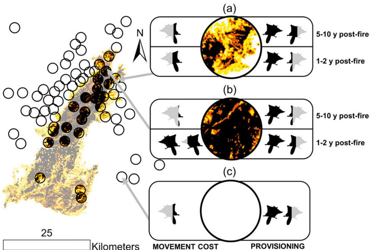
Fig. 6 Predicted movement costs and provisioning for historical spotted owl territories. We show predicted movement cost and energetic provisioning for three territories as the number of average sized flying squirrels (170 g) necessary per day which would satisfy those requirements. Solid black images represent 1 flying squirrel required per day, and partial images represent a proportion of a flying squirrel required per day. We
