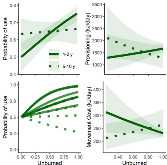
Fig. 4 Predicted effects of the proportion of unburned forest on resource selection, provisioning, and movement costs. Lines indicate predicted relationships between the proportion of unburned forest in capture polygons or home ranges and shaded areas indicate 95% confidence intervals. Solid lines show predicted relationships for sites burned 1–2 years prior and dotted lines show sites burned 5–10 years prior
