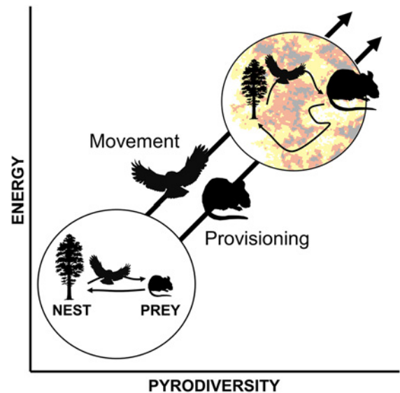
Fig. 1 Predicted relationship between pyrodiversity and energy. We expected that the energetic cost of movement, driven by distance traveled by owls, and energetic provisioning, driven by biomass of prey delivered to nests, would both increase with pyrodiversity at local and landscape scales
