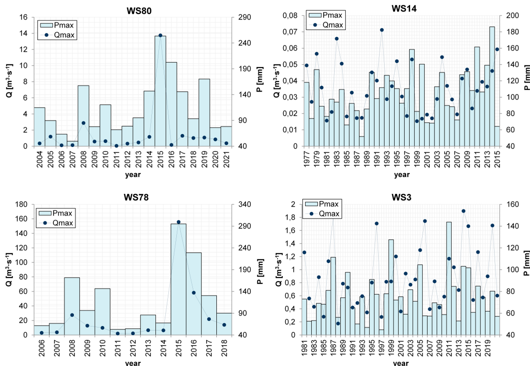
FIG. 2. Annual maxima time series for peak flow rates Q and daily precipitation P in the study catchments.
