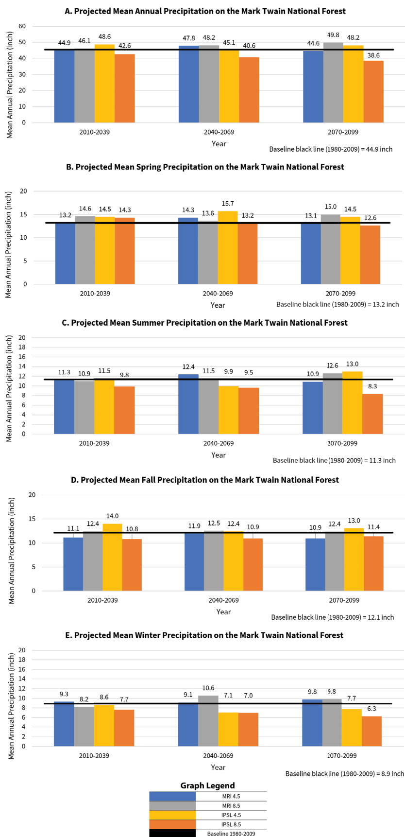
Figure 10. —Projected change in annual (A) and seasonal (B–E) precipitation under the four scenario combinations for three 30-year periods compared with the baseline period of 1980 through 2009 for the Mark Twain National Forest.
