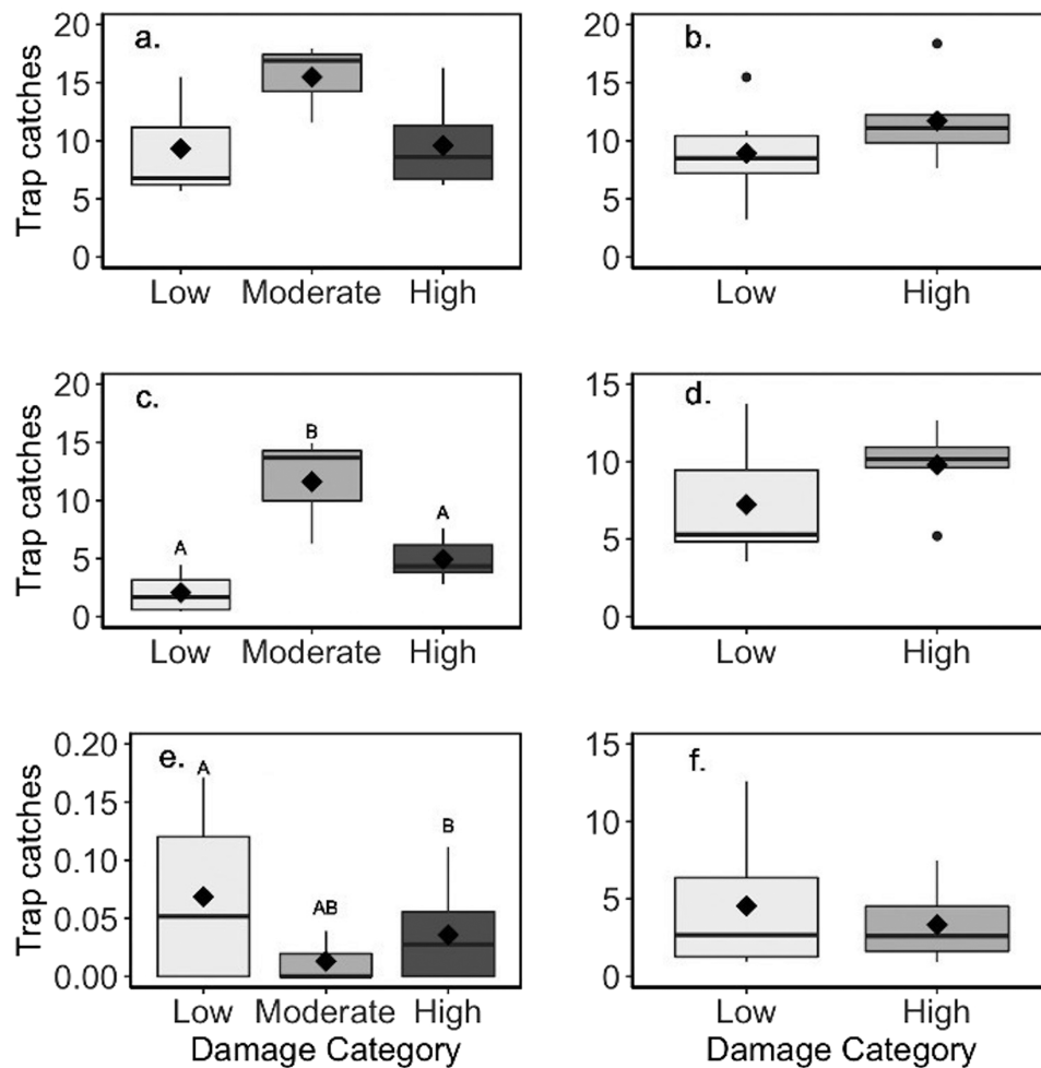
Figure 3 Boxplots depicting differences in means (diamonds), medians (horizontal lines), interquartile ranges (whiskers), and outliers (points) for standardized mean trap catches across damage categories for Acanthocinus obsoletus in (a) 2019 and (b) 2020, Monochamus spp. in (c) 2019 and (d) 2020, and Xylotrechus sagittatus in (e) 2019 and (f) 2020.
