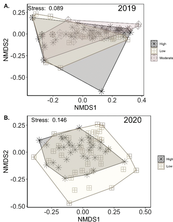
Figure 5 NMDS plots depicting Bray-Curtis dissimilarities in woodborer beetle assemblage composition among stand damage classes in (a) 2019 and (b) 2020.
