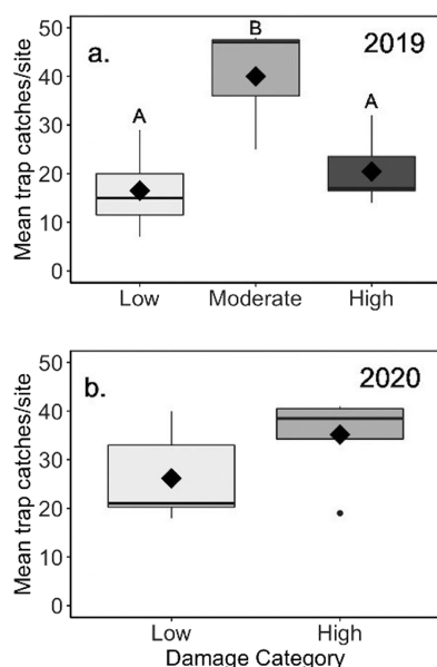
Figure 2 Boxplots depicting differences in means (diamonds), medians (horizontal lines), interquartile ranges (whiskers), and outliers (points) for total standardized mean trap catches across damage categories in (a) 2019 and (b) 2020.
