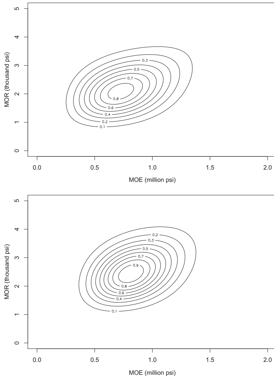
Figure 1.—Contour plots of two scaled Olkin & Liu Bivariate Beta densities from the database: BB_s(6.63, 5.44, 10.63, 2.42, 5.54) (top), and BB_s(6.69, 8.33, 16.36, 2.99, 6.31) (bottom).
